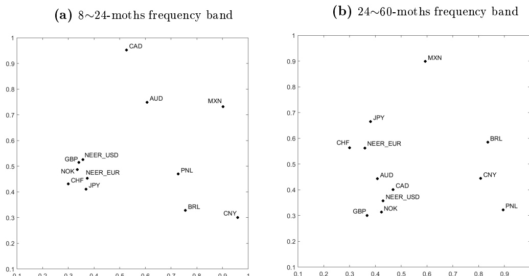
Figure 4: Multidimensional Scaling Maps
