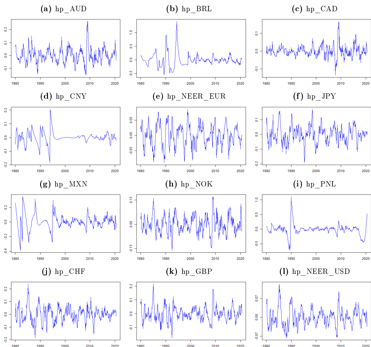
Figure 2: Cyclical components of the exchange rates
