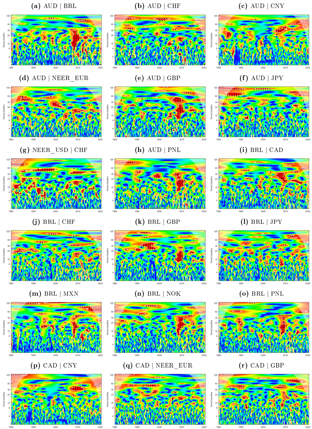
Figure 6: Cross-Wavelet Coherencies and Phase-Differences
