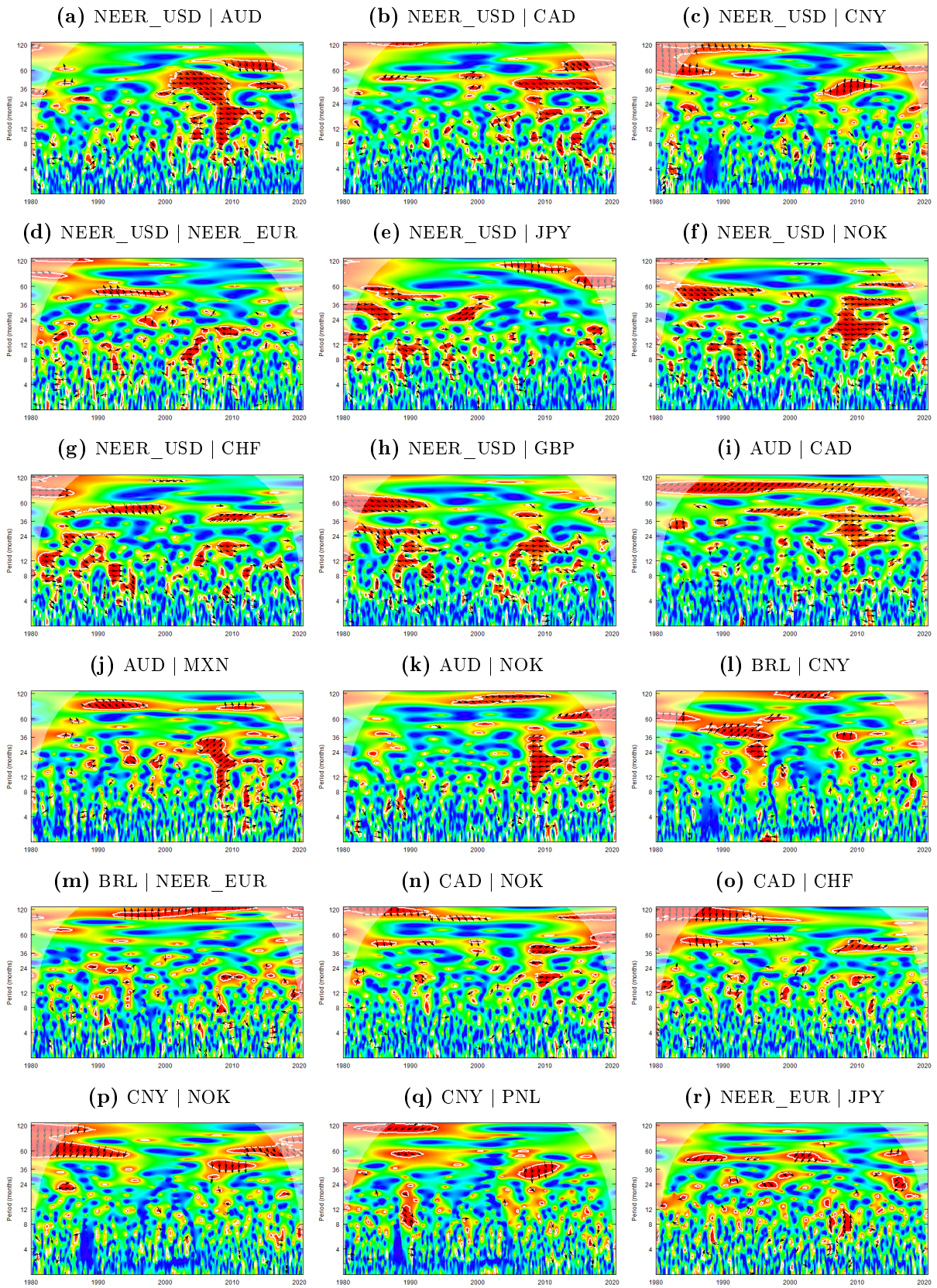
Figure 5: Cross-Wavelet Coherencies and Phase-Differences
