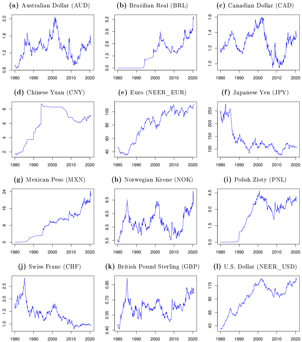
Figure 1: Nominal Exchange Rates
