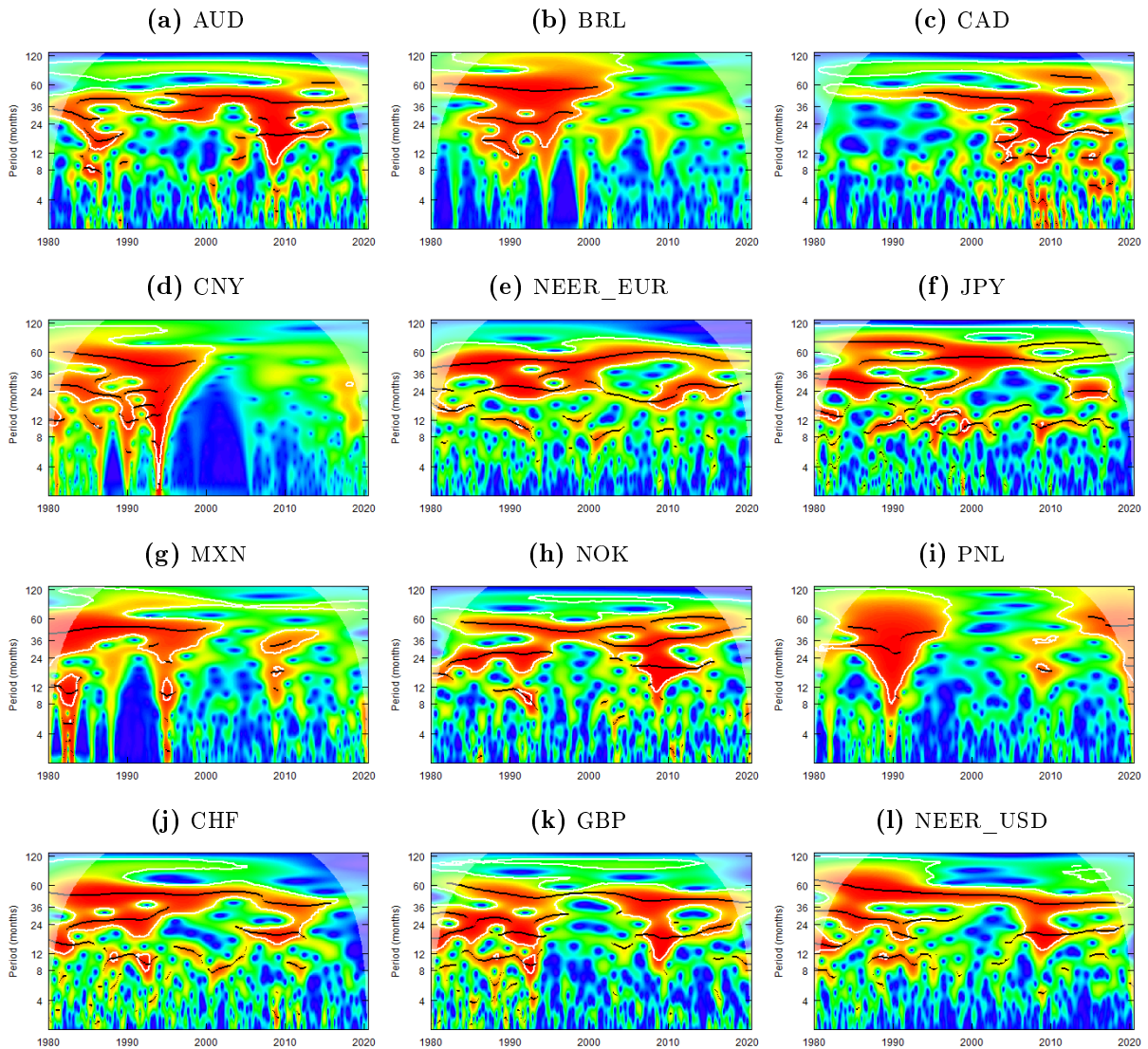
Figure 3: Wavelet Power Spectra
