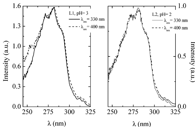
Figure 6. Fluorescence excitation spectra of compounds L1 and L2 in water at acidic pH values collected in the monomer ( \lambda_{em} = 330 nm) and excimer emission regions ( \lambda_{em} = 400 nm).
