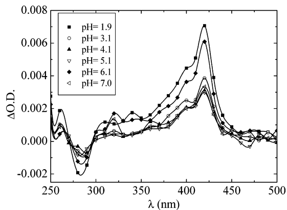
Figure 12. Transient triplet–triplet absorption spectra for compound L1 obtained at different pH values, T = 20^\circ\text{C} and delay after flash is 2\ \mu\text{s} .
