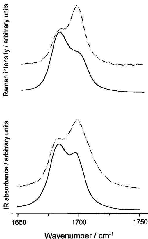
Figure 5. Room-temperature Raman and FTIR spectra of pure 4MeOB (solid line) and diluted 4MeOB, x = 0.1 in CCl 4 (dashed line), in the region of the C=O stretching modes.
