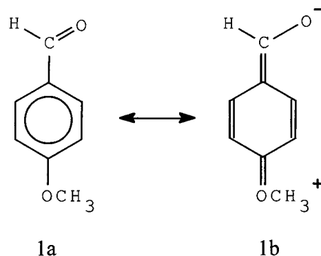
Figure 1. Chemical structure of 4MeOB molecule (a) showing the resonance structure with charge transfer from the methoxy group to the aldehyde group (b).
