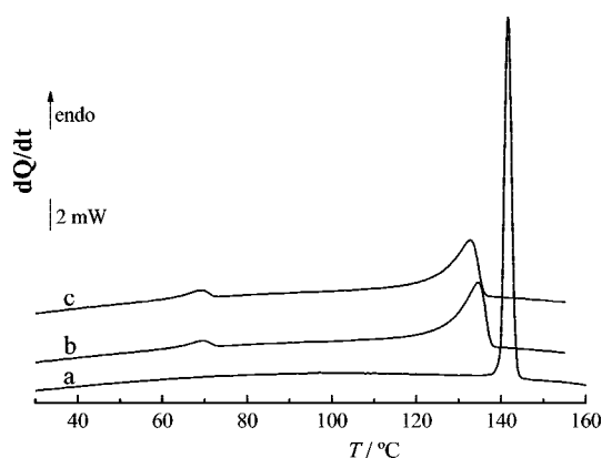
Figure 5. DSC heating curves obtained in heating/cooling cycles of ABIOD: (a) first heating run; (b) second heating run; (c) third heating run; m = 2.64 mg; heating rate 10 ^{\circ}\text{C min}^{-1} .
