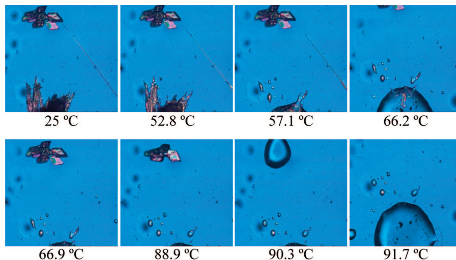
Figure 4. Fusion process of ABIOD observed by polarized light thermomicroscopy. Samples prepared by annealing at room temperature, for 30 days, the liquid obtained in the heating process of ABIOD. Magnification 200 \times . Heating rate 10 ^{\circ}\text{C min}^{-1} .
