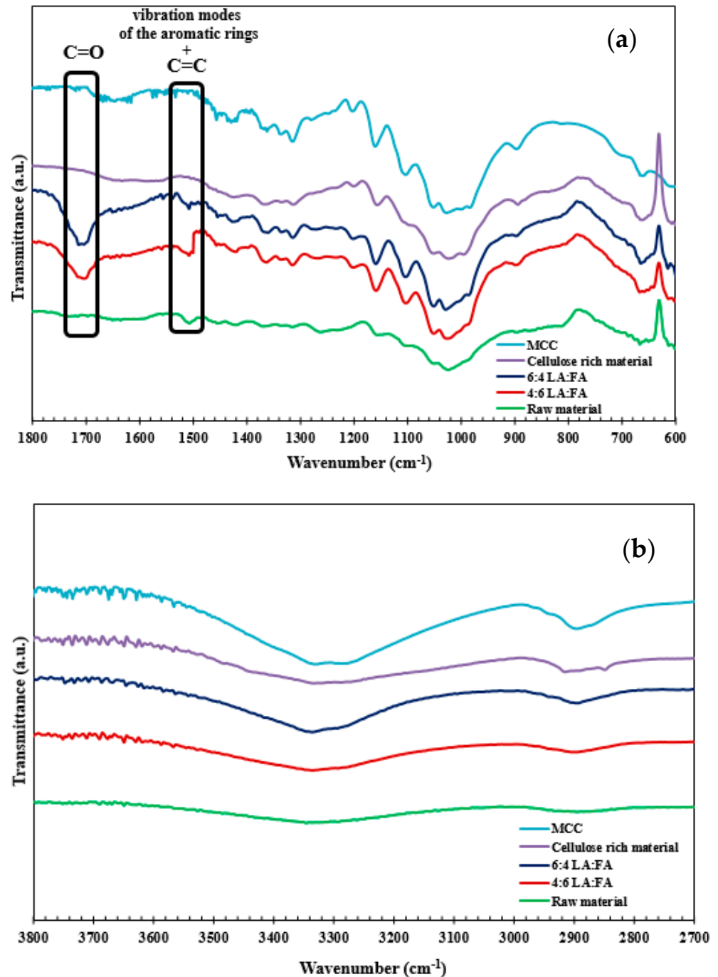
Figure 8. FTIR spectra for low (a) and high (b) wavenumbers of pre-extracted pine sawdust (raw material), the lignin obtained from the fractionation with 4:6 LA:FA (4 h at 160 °C), the lignin obtained from the fractionation with 6:4 LA:FA (4 h at 160 °C), cellulose-rich material obtained from the fractionation of pine sawdust with 6:4 LA:FA and “model” microcrystalline cellulose (MCC) from a commercial supplier.
