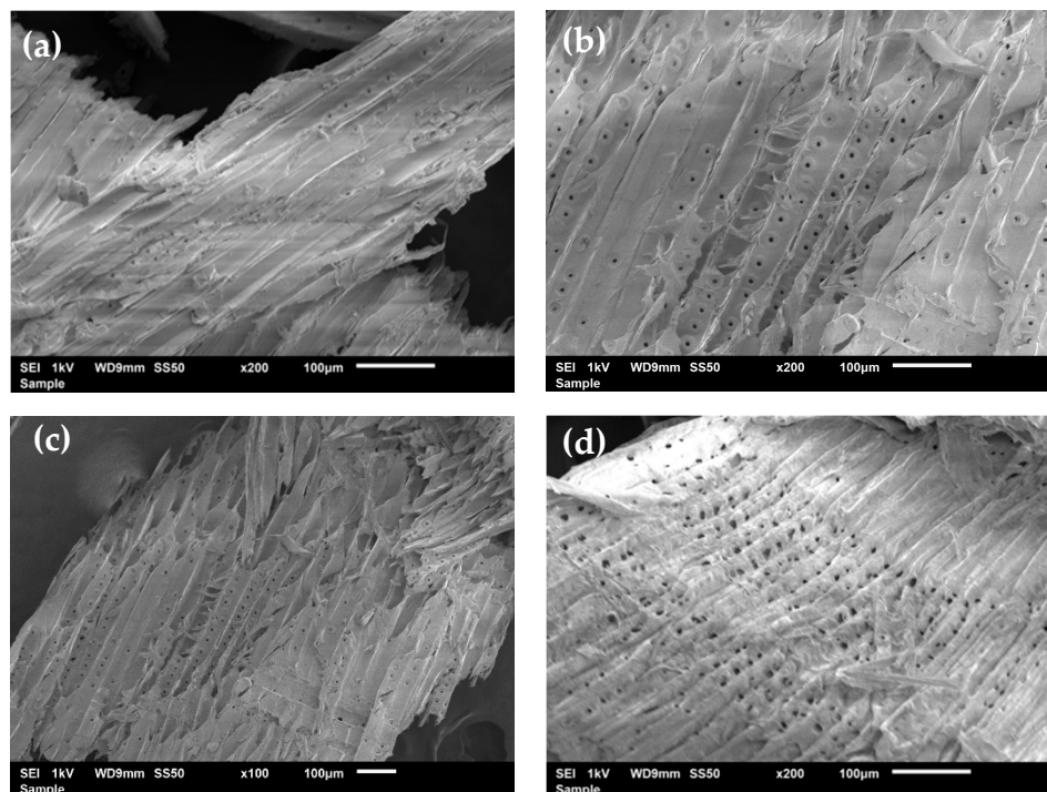
Figure 7. Scanning electron microscopy of the starting pine sawdust (a), and the cellulose-rich materials obtained after fractionation with 6:4 LA:FA lasting (b) 2 h at 160 °C, (c) 2 h at 120 °C, and (d) 4 h 160 °C.
