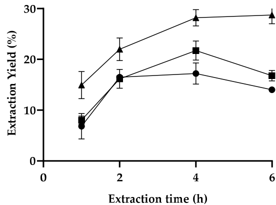
Figure 1. Extraction yield of LA:FA (1:1) as a function of extraction time for 120 °C (●), 140 °C (■) and 160 °C (▲).
