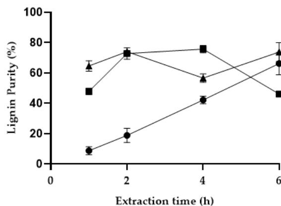
Figure 2. Purity of the lignin obtained by fractionation of the pine sawdust with the 1:1 LA:FA solvent system at different extraction times and temperatures, 120 °C (●), 140 °C (■) and 160 °C (▲).
