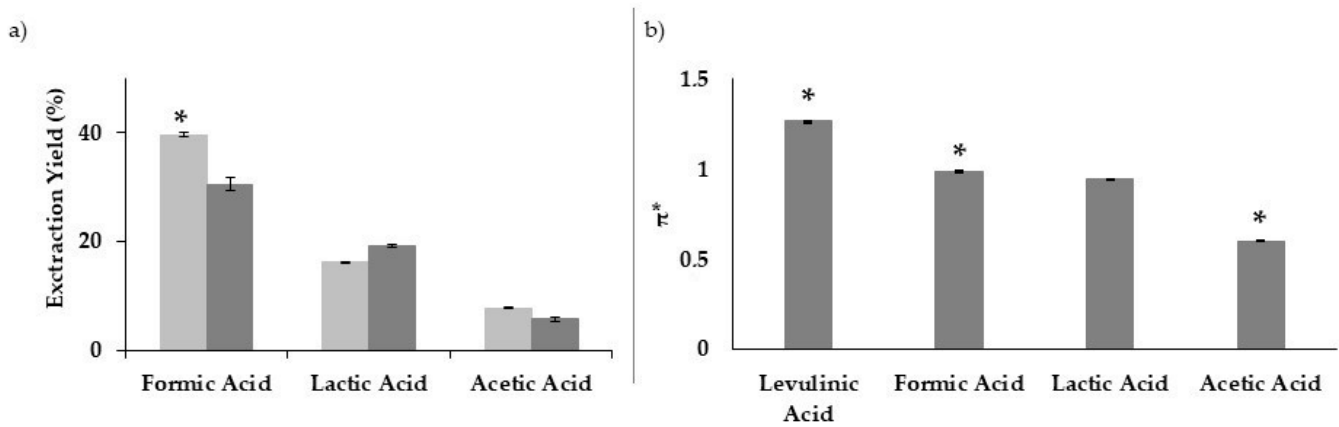
Figure 6. Extraction yield and polarization index \pi^* : (a) effect of different acids on the extraction yield of solvent mixtures containing either 6:4 of LA:acid (dark grey) or 4:6 LA:acid (light grey), for 2 h at 160 °C; (b) \pi^* values for different acids. The same symbols above the bars indicate no significant differences in the extraction yield and in the lignin purity (Figure 6a) and \pi^* values (Figure 6b) from one-way ANOVA tests ( p \leq 0.05 ).
