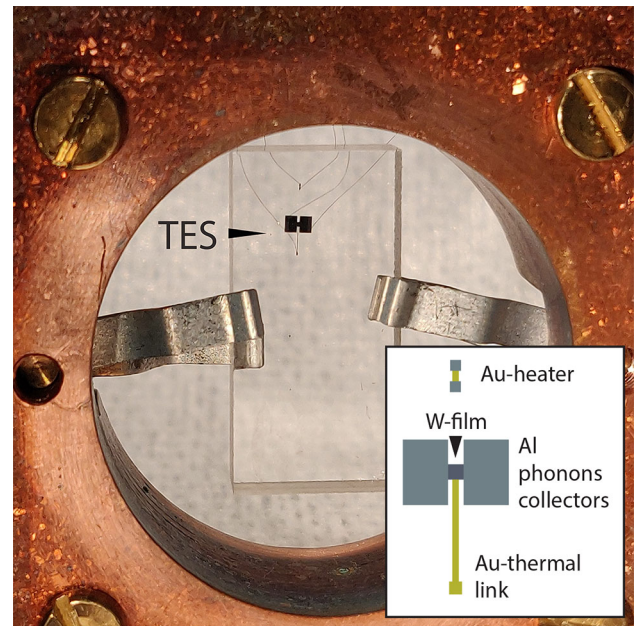
Fig. 2 Close-up of module B , constituted by a 2.8 g \text{LiAlO}_2 crystal instrumented with a TES directly deposited on the surface. On the bottom right corner a scheme of the TES is shown (see text for details)
