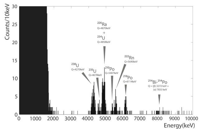
Fig. 12 Energy spectrum registered by the NTD during a background measurement of 35.6 h effective time. From this spectrum at least seven different sources of \alpha decays in the 4–7 MeV region can be distinguished and above 7 MeV additional events, likely due to {}^{214}\text{Bi} – {}^{214}\text{Po} decays, appear
