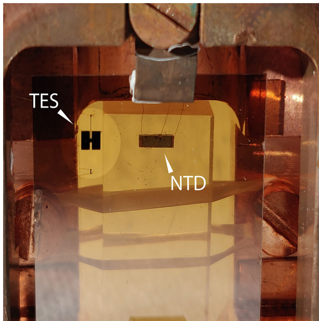
Fig. 1 Close-up of module A . It is possible to see the 2.8 g \text{LiAlO}_2 crystal instrumented with the NTD sensor through the CRESST-III light detector
