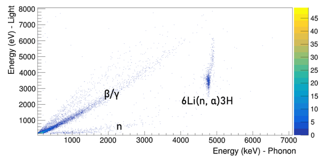
Fig. 5 Energy measured by the CRESST-III light detector versus energy measured by the NTD for each event registered by module A in the presence of an AmBe neutron source during 9.44 hours of data collection. Two bands starting from zero appear: the one with the higher light emission is constituted by \beta/\gamma events interacting inside the \text{LiAlO}_2 crystal, while the one with lower light emission is caused by the scattering of neutrons within the crystal. At 4780 keV a different family of events appears, due to the neutron capture of ^6\text{Li} . In the vicinity of the neutron capture there is an additional family of events, with a slightly higher energy. This family currently is of unknown origin and the modeling of the anomalously high light yield is particularly challenging
