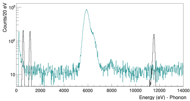
Fig. 7 Energy spectrum collected during 22.2 h of background measurement with module B without any cut applied to the data set. In black: events induced by injected heater pulses. In light blue: particle events only. At 5.895 keV the peak caused by the X-ray emission of ^{55}\text{Fe} decay appears; the energy resolution at 5.895 keV is equal to \sigma_{K_\alpha} = (184.0 \pm 1.6) eV. The resolution for heat pulse events is equal to \sigma_{HP_2} = (41.6 \pm 1.0) eV at 1.159 keV and \sigma_{HP_3} = (57.0 \pm 1.6) eV at 11.537 keV. Below 300 eV there is a rise in the spectrum
