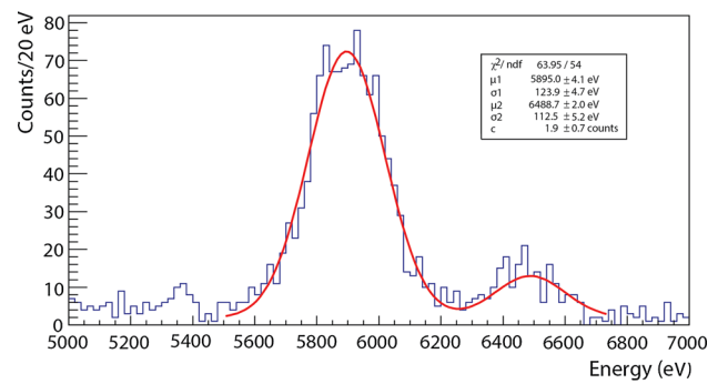
Fig. 4 Energy spectrum of events registered by the CRESST-III light detector in the energy region of X-ray emission by the ^{55}\text{Fe} source. Two peaks are visible: one at 5.895 keV, resulting from the sum of K_{\alpha 1} and K_{\alpha 2} lines, and one at 6.490 keV, resulting from the sum of K_{\beta 2} and K_{\beta 3} lines. The fit function (red solid line) consists of the sum of two Gaussian functions ( \mu_1 and \mu_2 are the expected values, \sigma_1 and \sigma_2 the standard deviations) plus a constant factor c to account for the flat background. In principle, \sigma_2 should not be lower than \sigma_1 , but we attribute this anomaly to the presence of an energy loss in the left shoulder of the 5.895 keV peak. The 5.895 keV peak is used to obtain the energy calibration of the light detector
