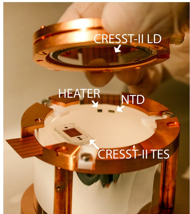
Fig. 9 Detector module C was operated at LNGS. A 373 g crystal is instrumented with two phonon sensors glued on the top surface: an NTD and a CRESST-II TES. On the same surface there is a glued heater which ensures the stability of the detector operation. The crystal is surrounded by reflective foil and a CRESST-II light detector is facing the top surface of \text{LiAlO}_2
