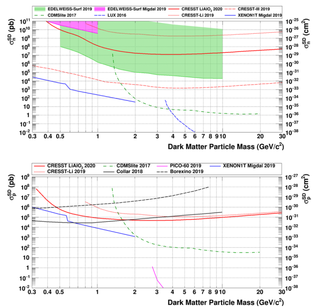
Fig. 8 Top: Exclusion limits set by various direct detection experiments for spin-dependent interactions of dark matter particles with neutrons. The result obtained from module B data with ^7\text{Li} + ^{27}\text{Al} is shown in solid red. The first result obtained by CRESST using ^7\text{Li} is plotted in dotted red [5], while the result obtained with ^{17}\text{O} in CRESST-III is shown in dashed red [4]. For comparison, limits from other experiments are also shown: EDELWEISS [34] and CDMSlite [35] using ^{73}\text{Ge} , LUX [36] and XENONIT (Migdal effect) [37] using ^{129}\text{Xe} + ^{131}\text{Xe} . Bottom: The same, but for spin-dependent interactions of dark matter particles with protons. The result obtained from module B data with ^7\text{Li} + ^{27}\text{Al} is shown in solid red. The first result obtained by CRESST using ^7\text{Li} is plotted in dotted red [5]. Additionally, limits from other experiments are also shown: CDMSlite with ^{73}\text{Ge} [35]; PICO with ^{19}\text{F} [38]; XENONIT (Migdal effect) with ^{129}\text{Xe} + ^{131}\text{Xe} [37]; Collar with ^1\text{H} [39]. Finally, a constraint from Borexino data derived in [40] is shown in dotted black
