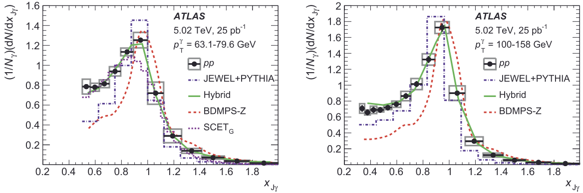
Fig. 9. Photon-jet p_T -balance distributions (1/N_\gamma)(dN/dx_{J\gamma}) in pp collisions for (left) p_T^\gamma = 63.1\text{--}79.6 \text{ GeV} and (right) p_T^\gamma = 100\text{--}158 \text{ GeV} . The unfolded results are compared with the theoretical calculations shown as dashed coloured lines (see text). Total systematic uncertainties are shown as boxes, while statistical uncertainties are shown as vertical bars.
