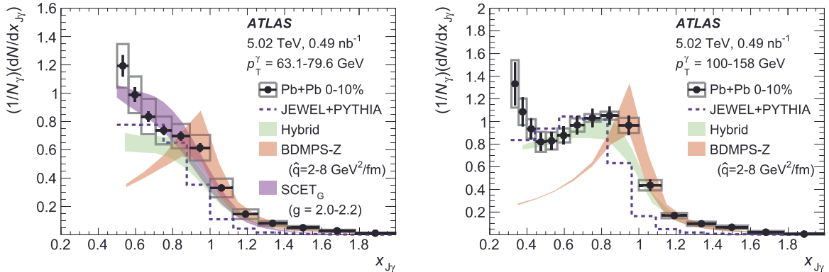
Fig. 10. Photon-jet p_T -balance distributions (1/N_\gamma)(dN/dx_{J\gamma}) in 0–10% Pb + Pb collisions for (left) p_T^\gamma = 63.1\text{--}79.6 \text{ GeV} and (right) p_T^\gamma = 100\text{--}158 \text{ GeV} . The unfolded results are compared with the theoretical calculations shown as dashed coloured lines denoting central values or coloured bands which correspond to a range of theoretical parameters (see text). Total systematic uncertainties are shown as boxes, while statistical uncertainties are shown as vertical bars.
