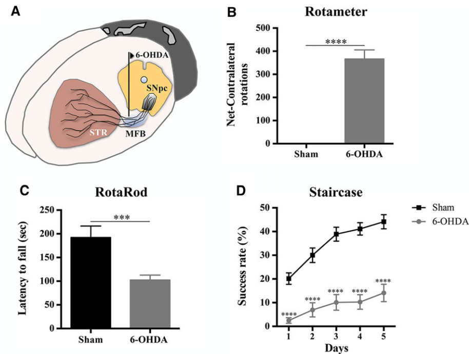
Figure 2. Behavioral characterization of 6-OHDA lesions. (A): The animals received unilateral injections of 6-OHDA directly in the MFB. (B): Rotameter revealed that the animals injected with 6-OHDA exhibited an intense turning behavior when compared to sham group. 6-OHDA-injected animals also presented significant impairment in motor coordination and balance (C) and in the paw-reaching test performance (D) . For the Rotameter test, n = 9 for sham group and n = 13 for 6-OHDA group. For the RotaRod test, n = 7 for sham group and n = 14 for 6-OHDA group. For the Staircase test, n = 9 for sham group and n = 15 for 6-OHDA group. Data are presented as mean \pm SEM. ***p \leq .001 ; ****p \leq .0001 . Abbreviations: 6-OHDA, 6-hydroxidopamine; MFB, medial forebrain bundle; sec, seconds; SNpc, substantia nigra pars compacta; STR, striatum.
