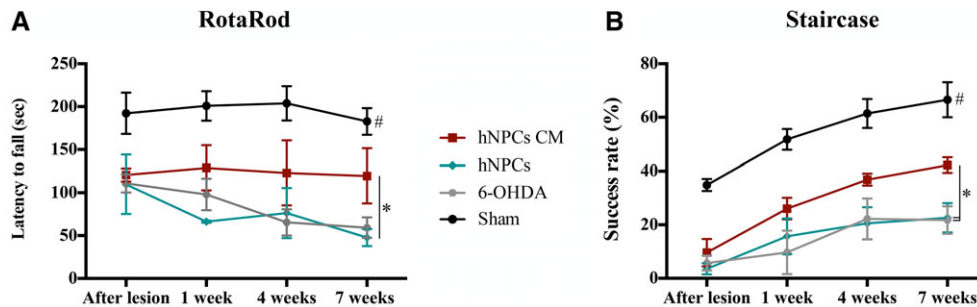
Figure 3. Behavioral characterization 1, 4, and 7 weeks after hNPCs transplantation and hNPCs CM (i.e., secretome) injection in the SNpc and striatum. (A): Latency to fall was measured in the accelerating RotaRod test, demonstrating that the hNPCs CM-injected animals had a statistical significant improvement in their motor coordination when compared to the hNPCs-transplanted group (at 7 weeks after injection). (B): The Staircase test also demonstrated a statistical significant improvement of the forelimb coordination of the hNPCs CM-injected animals when compared to both the untreated group 6-OHDA and the hNPCs-transplanted group (at 7 weeks after injection). For the RotaRod test, n = 7 for sham group, n = 5 for 6-OHDA group, n = 5 for hNPCs transplanted group and n = 5 for hNPCs CM-injected animals. For the Staircase test, n = 9 for sham group, n = 5 for 6-OHDA group, n = 5 for hNPCs transplanted group and n = 5 for hNPCs CM-injected animals. Data are presented as mean \pm SEM. *p \leq .05 ; Sham animals statistically different from all the other groups: \# p \leq .0001 . Abbreviations: 6-OHDA, 6-hydroxidopamine; hNPCs, human neural progenitor cells; hNPCs CM, human neural progenitor cells-conditioned media; SNpc, substantia nigra pars compacta.
