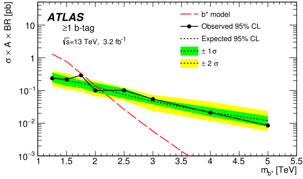
Fig. 5. Observed (filled circles) and expected (dotted line) 95% credibility-level upper limits on the cross section \sigma times acceptance A times branching ratio BR , including kinematic acceptance and b -tagging efficiencies, for the b^* model. The dashed line shows the cross section calculated from theory. The plot shows the case with a single b -tag.
