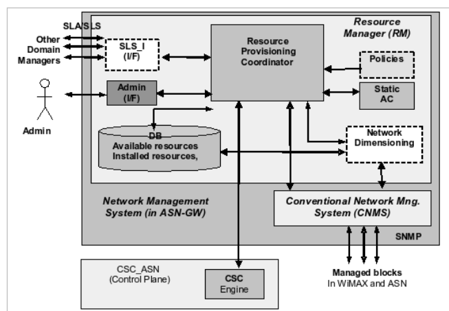
Fig. 3. WEIRD Management Plane.
