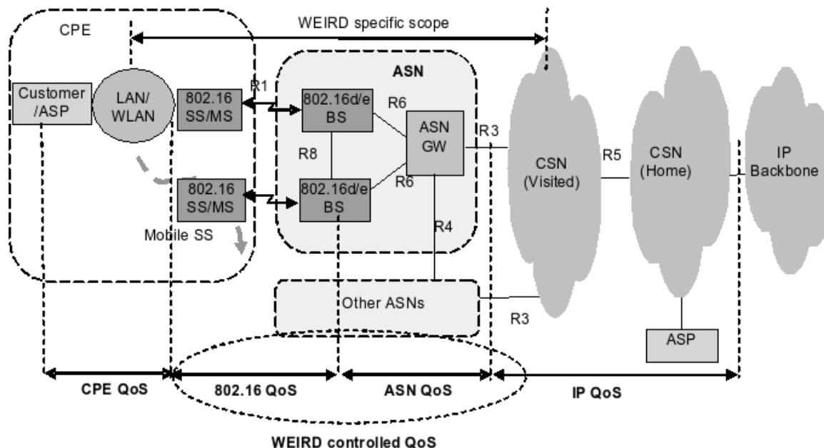
Fig. 1. Simplified WEIRD Overall Network Infrastructure
