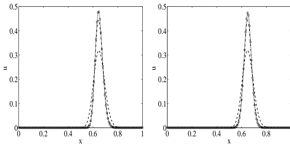
FIGURE 11. Approximated solution for u = 0.5 , D = 0.001 and \Delta x = 0.008 k = 0 (---); k = 1 (- · -); k = 2 (- o -) (a) Classical Mpdata (b) Third-order Mpdata
