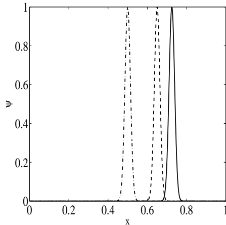
FIGURE 2. Initial solution ( - \cdot - ). Exact solution at t = 0.3 for u = 0.5 ( - ) and for u = 0.75 ( - \cdot - )
