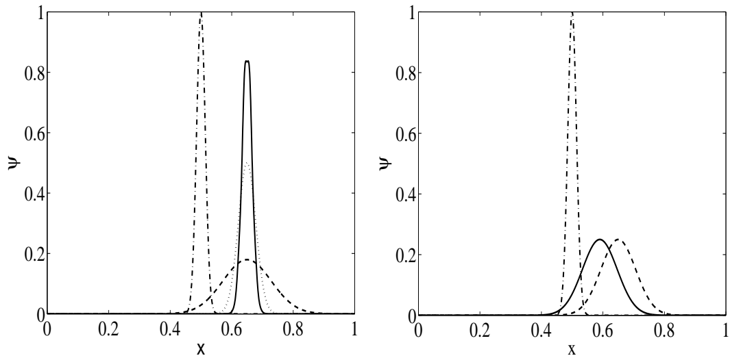
FIGURE 6. Initial solution ( - \cdot - ). Exact solution at t = 0.3 for: (a) u = 0.5 D = 0.01 ( -- ); u = 0.5 D = 0.001 ( \cdot \cdot \cdot ); u = 0.5 D = 0.0001 ( - ). (b) u = 0.5 D = 0.005 ( - ); u = 0.3 D = 0.005 ( -- )
