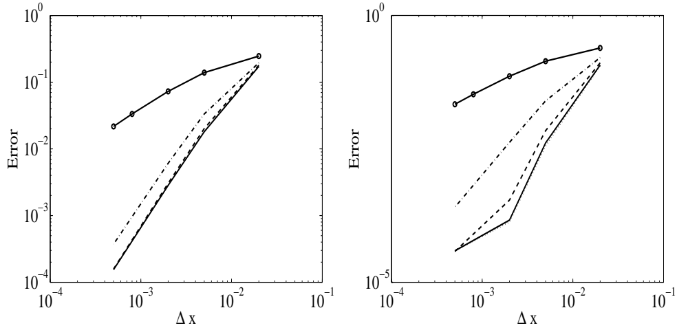
FIGURE 7. Error function as mesh is refined for: k = 0 , (-o-) ; k = 1 , (-\cdot-\cdot-) ; k = 2 (--) ; k = 3 (-) ; k = 4 (\cdot\cdot\cdot) . u = 0.5 , D = 0.001 (a) Classical Mpdata (b) Third-order Mpdata. Order of convergence in Table 6.
