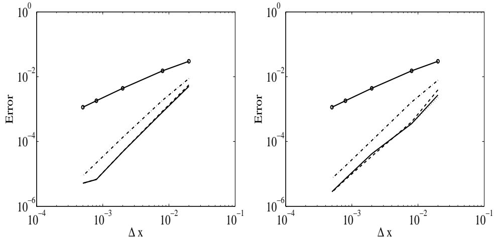
FIGURE 8. Error function as mesh is refined for: k = 0 , (-o-) ; k = 1 , (-\cdot-\cdot-) ; k = 2 (--) ; k = 3 (-) ; k = 4 (\cdot\cdot\cdot) . u = 0.5 , D = 0.01 (a) Classical Mpdata (b) Third-order Mpdata. Order of convergence in Table 5.
