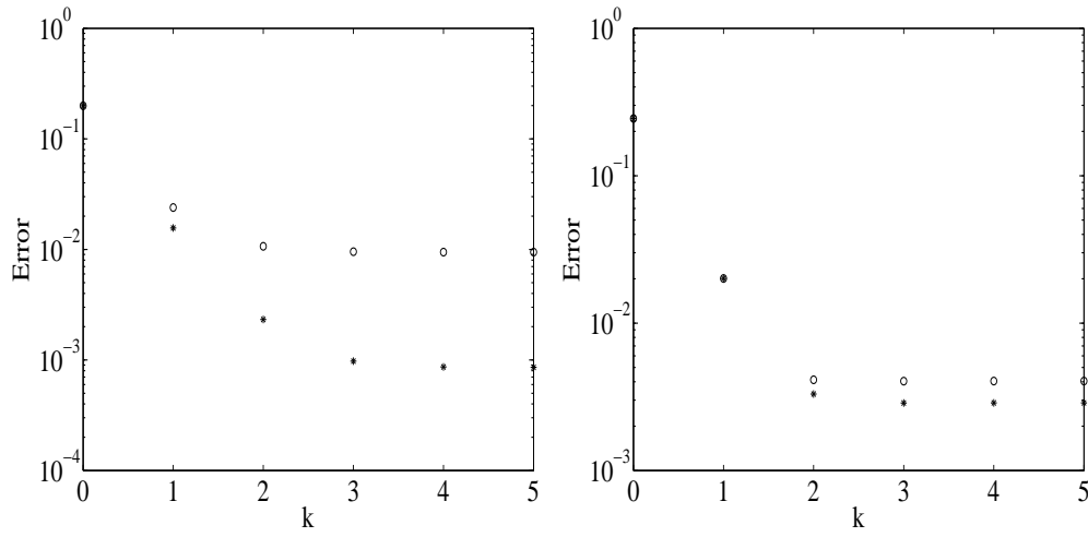
FIGURE 5. Error function as k increases: \Delta x = 0.002 Classical Mpdata ( o ); Third-order Mpdata ( * ) (a) u = 0.75 (b) u = 0.5
