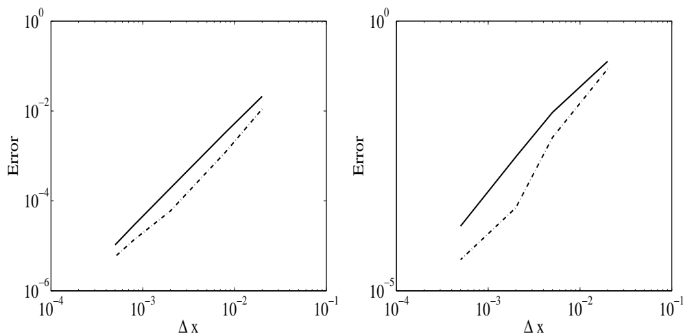
FIGURE 10. Error versus space step for Classical Mpdata ( - ) and Third-order Mpdata ( - \cdot - ) and k = 2 . (a) u = 0.5 , D = 0.005 . Same order of accuracy but smaller error for the Third-order Mpdata. (b) u = 0.5 , D = 0.001 . High-order accuracy for the Third-order Mpdata
