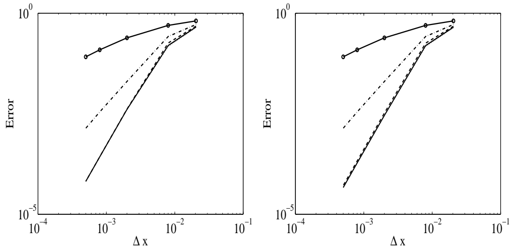
FIGURE 3. Error function as mesh is refined for: k = 0 , (-o-) ; k = 1 , (-\cdot-) ; k = 2 (--) ; k = 3 (-) ; k = 4 (\cdot\cdot\cdot) . u = 0.5 (a) Classical Mpdata (b) Third-order Mpdata
