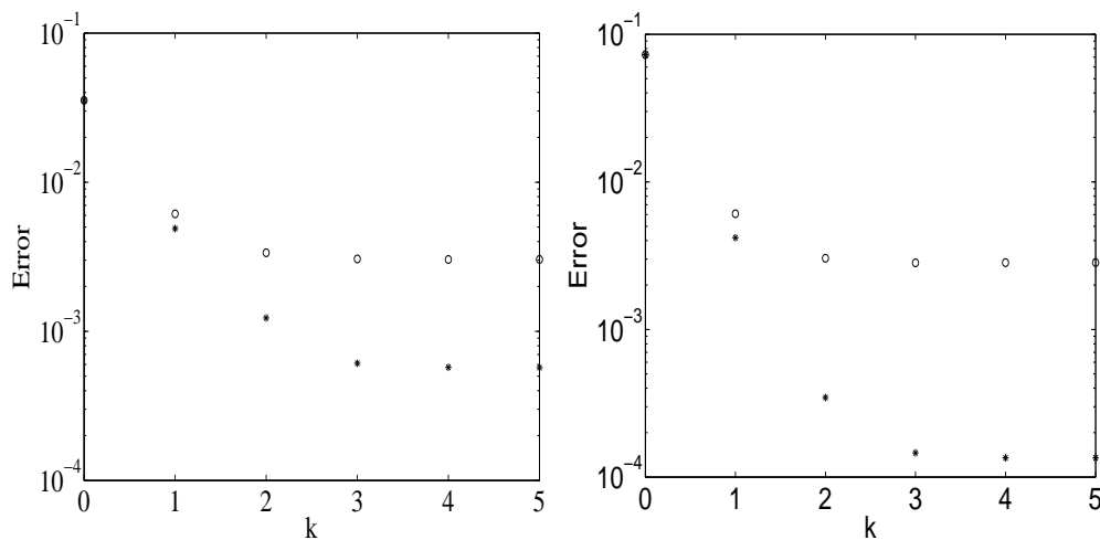
FIGURE 9. Error function as k increases: Mpdata classical ( o ); Mpdata third-order ( * ) (a) u = 0.5 D = 0.005 \Delta x = 0.008 ; (b) u = 0.5 D = 0.001 \Delta x = 0.002
