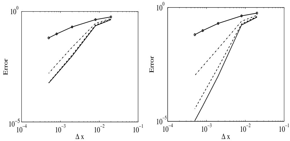
FIGURE 4. Error function as mesh is refined for: k = 0 , (-o-) ; k = 1 , (-\cdot-) ; k = 2 (--) ; k = 3 (-) ; k = 4 (\cdot\cdot\cdot) . u = 0.75 (a) Classical Mpdata (b) Third-order Mpdata
