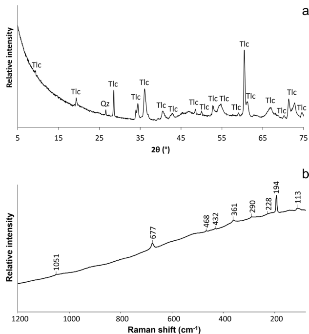
Fig. 2 Results of the μ-XRD and micro-Raman spectroscopy analysis of the type 44 bead found in Lumbu (Mbanza Kongo, Angola). a diffractogram identifying talc (Tlc) and quartz (Qz) as main constituents. b Raman spectra with marked Raman bands that are attributable to talc
