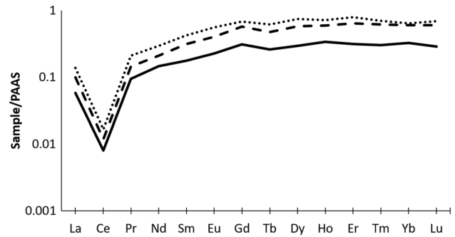
Fig. 4 PAAS-normalized REE pattern of the three measurements performed on the type 44 bead found in Lumbu (Mbanza Kongo, Angola). Significant Ce anomaly should be noted
