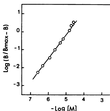
Fig. 5. Hill plot analysis of Tx binding to CaM. The plot was performed with the results ( \text{Ca}^{2+} -dependent binding) depicted in Fig. 4.
