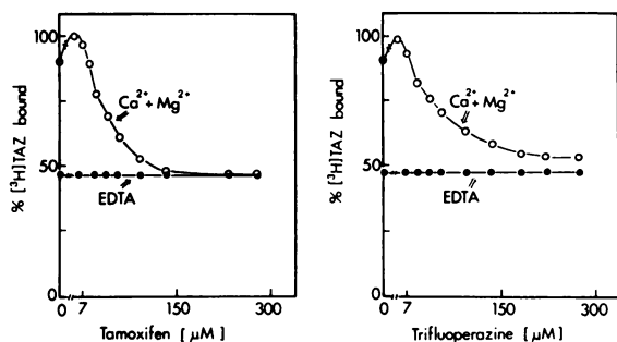
Fig. 6. Competition between [ ^3\text{H} ]TAZ and nonradiolabeled Tx or trifluoperazine for \text{Ca}^{2+} -dependent Tx binding sites of CaM. CaM (15 \mu\text{g} ) was incubated 1 h at 25°C with various concentrations (0.1–260 \mu\text{M} ) of Tx or trifluoperazine, in a medium containing \text{Ca}^{2+} plus \text{Mg}^{2+} (0.1 mM plus 5 mM) or EDTA (5 mM) and 8 nM [ ^3\text{H} ]TAZ, in a buffer solution as described in Fig. 1. The unbound ligands were removed by the DCC technique as described in "Materials and Methods." Left , competition between [ ^3\text{H} ]TAZ and unbound Tx; right , competition between [ ^3\text{H} ]TAZ and trifluoperazine. O, presence of \text{Ca}^{2+} , ●, absence of cations (EDTA present).
