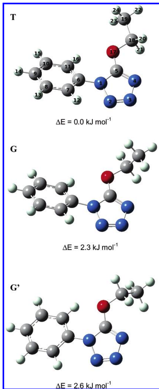
Figure 1. Optimized structures for the 5-ethoxy-1-phenyl-1H-tetrazole conformers T , G , and G' (with atom numbering). Relative energies calculated at the B3LYP/6-311++G(d,p) level of theory are also given (with zero point correction). Absolute calculated energy for conformer T is equal to -1\,689\,043.2 \text{ kJ mol}^{-1} . Atoms 1–4 are nitrogens, and atom 17 is oxygen.
