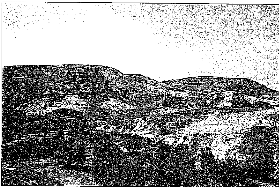
Fig. 4 - General view of Lower-Middle Toarcian marl-limestone alternations (S. Gião Formation) in the Rabaçal region.
