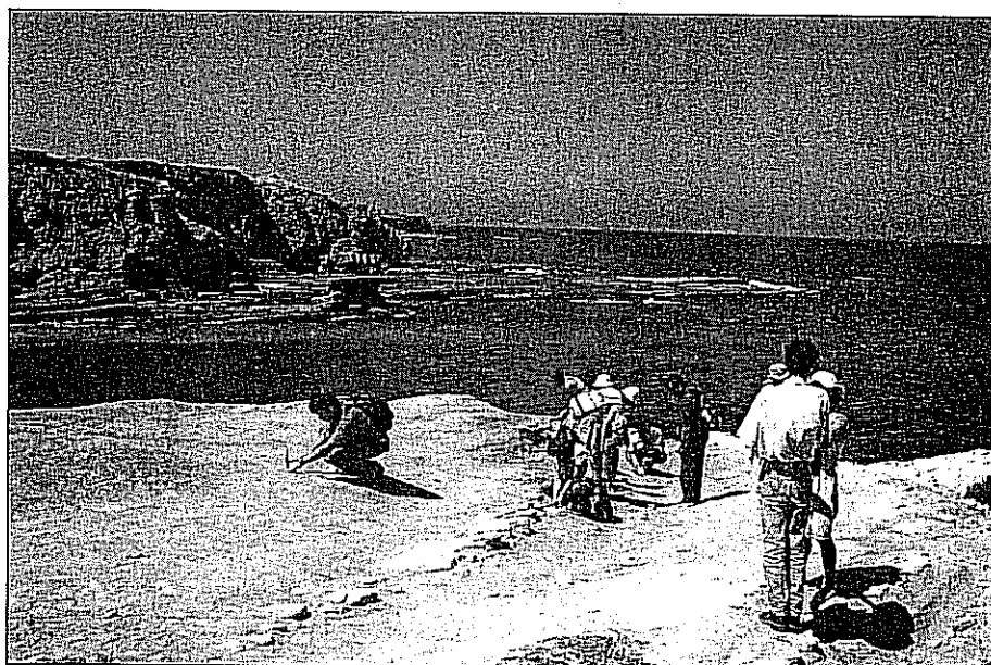
Fig. 5 - Partial view of Lower Toarcian succession in the Peniche Peninsula.
