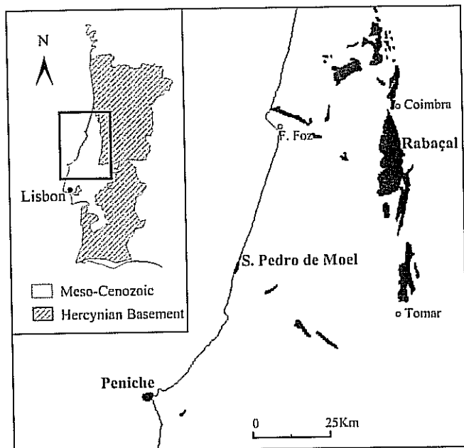
Fig. 1 - Main Lower Jurassic outcrops in the Lusitanian Basin, to the north of Lisbon. Location of the proposed geosites.
