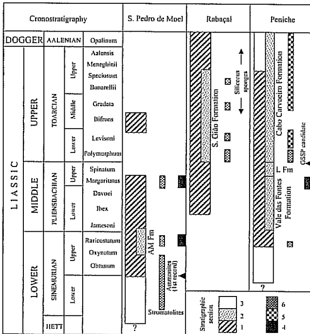
Fig. 2 - Stratigraphic range and main features of S. Pedro de Moel, Rabaçal and Peniche sections. Legend: 1 - High biostratigraphic control; 2 - Formation type-section (AM Fm - Água de Madeiros Formation; L Fm - Lemedo Formation); 3 - Without biostratigraphic data; 4 - Anoxic facies; 5 - Siliciclastic and/or oolitic facies; 6 - Highly fossiliferous levels (high vulnerability).
