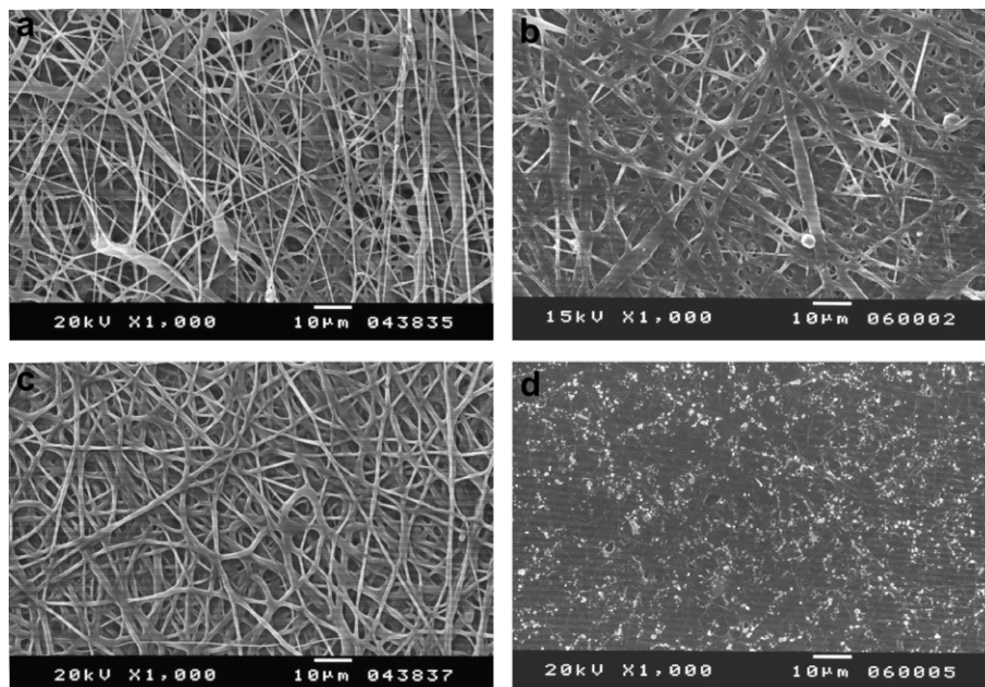
Fig. 2. Fibers a) PCL as prepared, b) PCL degraded during 12 months, c) 50/50 Lu/PCL as prepared, d) 50/50 Lu/PCL degraded during 12 months.
