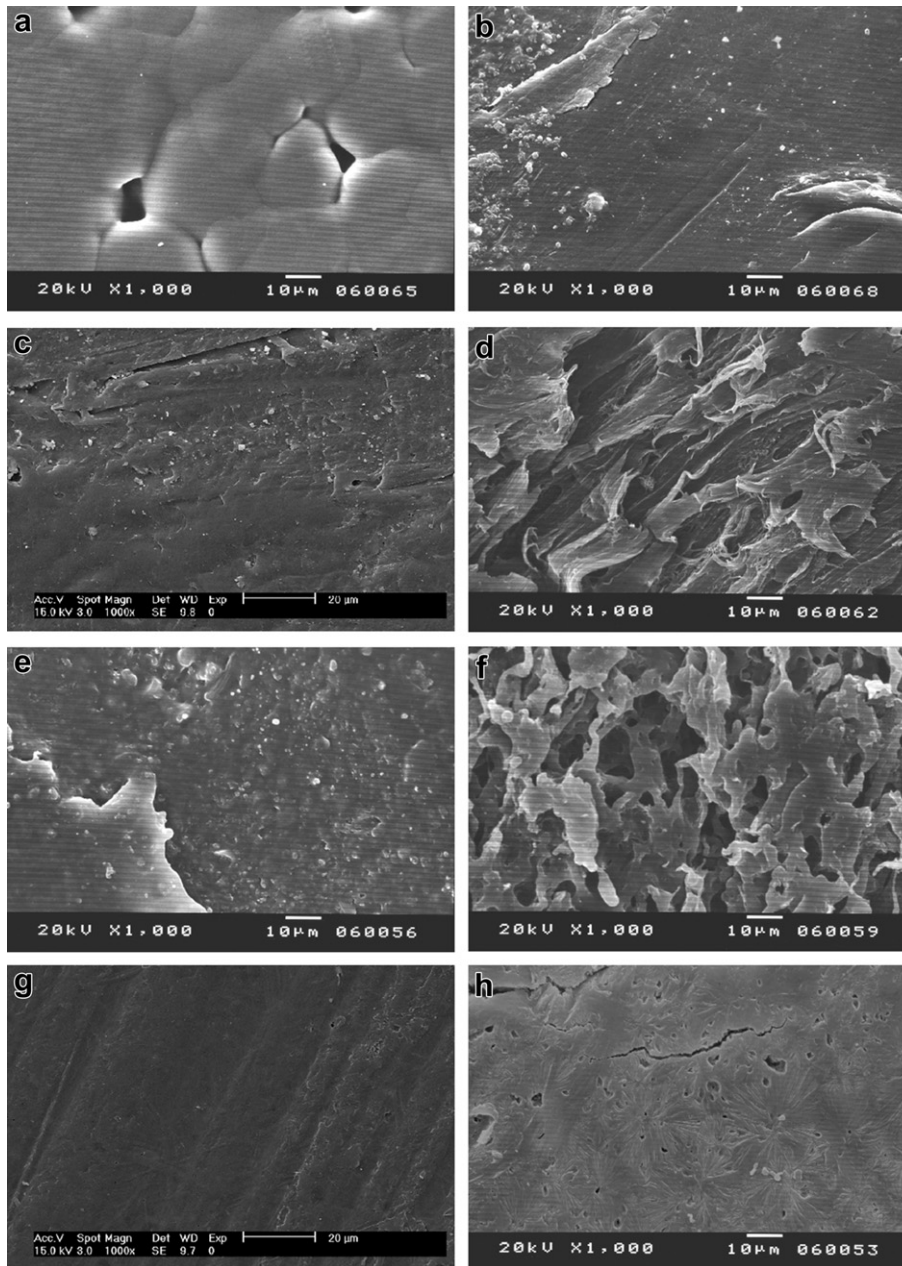
Fig. 4. Disks a) PCL as prepared, b) PCL degraded during 12 months, c) PCL + drug as prepared, d) PCL + drug degraded during 12 months, e) 50/50 Lu/PCL + drug as prepared, f) 50/50 Lu/PCL + drug degraded during 12 months, g) PCL10 + drug as prepared, h) PCL10 + drug degraded during 12 months.
