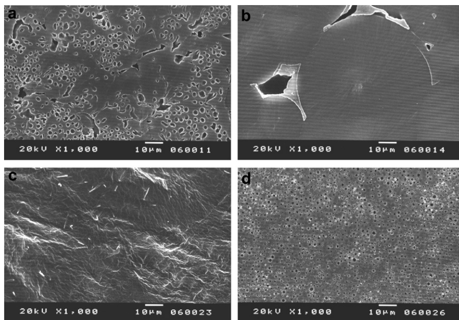
Fig. 1. Films a) PCL as prepared, b) PCL degraded during 12 months, c) 50/50 Lu/PCL as prepared, d) 50/50 Lu/PCL degraded during 12 months.
