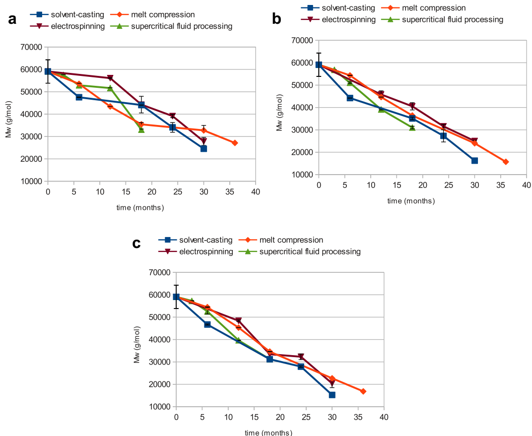
Fig. 5. Weight-average molecular weight of a) PCL, b) 25/75 Lu/PCL and c) 50/50 Lu/PCL constructs.
