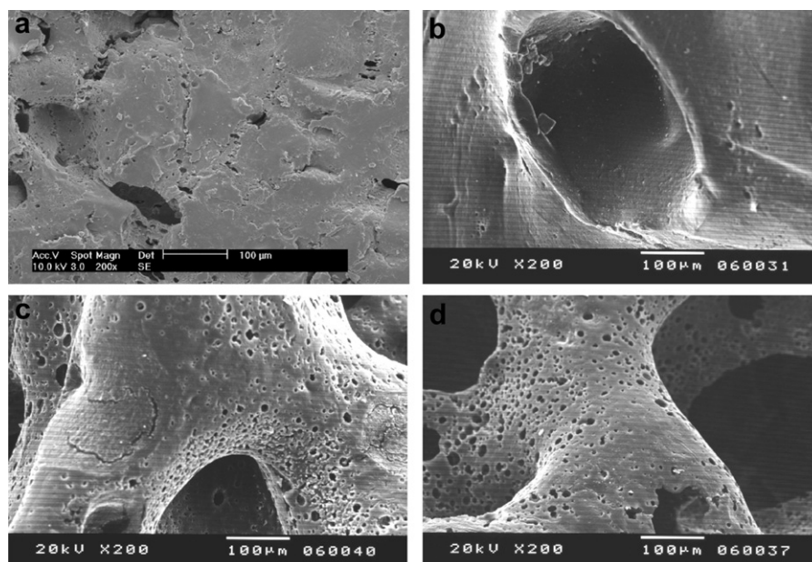
Fig. 3. Sponges a) PCL as prepared, b) PCL degraded during 12 months, c) 50/50 Lu/PCL as prepared, d) 50/50 Lu/PCL degraded during 12 months.
