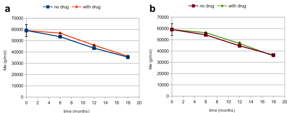
Fig. 7. Weight-average molecular weight of a) PCL, b) 25/75 Lu/PCL disks.
