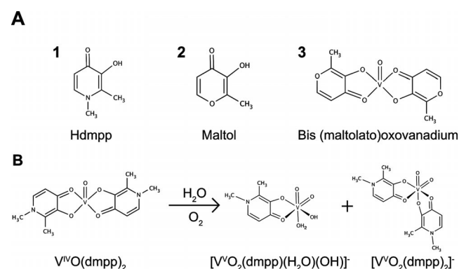
Scheme 1. A) Chemical structures of 3-hydroxy-1,2-dimethyl-4-pyridinone ( 1 , Hdmpp), 3-hydroxy-2-methyl-4-pyridone ( 2 , Maltol) and bis(maltolato)oxovanadium(IV) ( 3 , BMOV) (with K_1 = 107.5 and K_2 = 106.2 ). B) Chemical equilibrium representing the dissolution of the solid bis[3-hydroxy-1,2-dimethyl-4-pyridinonato]oxovanadium(IV), [V^{IV}O(dmpp)_2] in H_2O under physiological conditions and the resulting oxidation products, the vanadium(V) species [VO_2(dmpp)(H_2O)(OH)]^- and [VO_2(dmpp)_2]^- , with M/L ratios of 1:1 and 1:2, respectively (with K_1 = 1010.48 and K_2 = 105.25 ).
