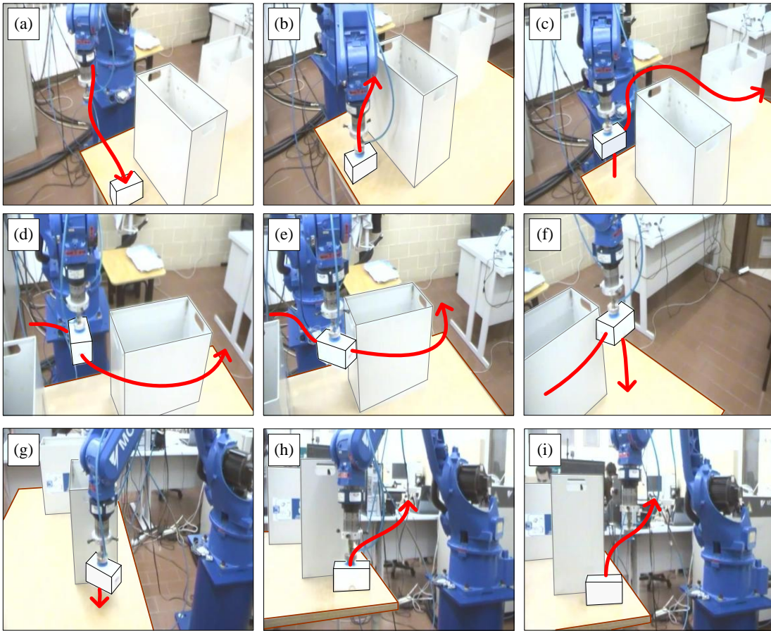
Fig. 25. Robot running the program generated from CAD.
