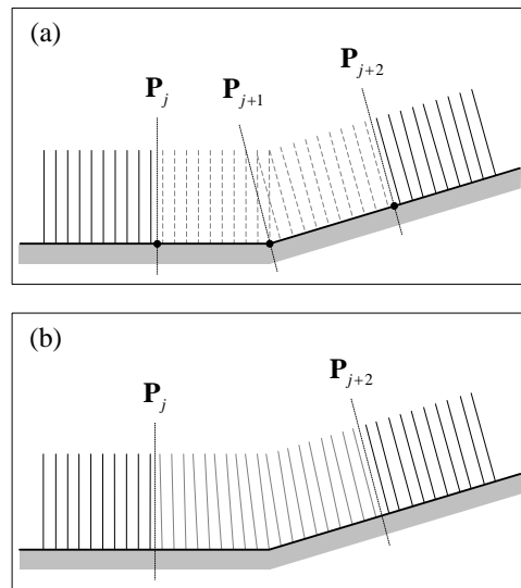
Fig. 16. End-effector poses: (a) before interpolation and (b) after interpolation.
