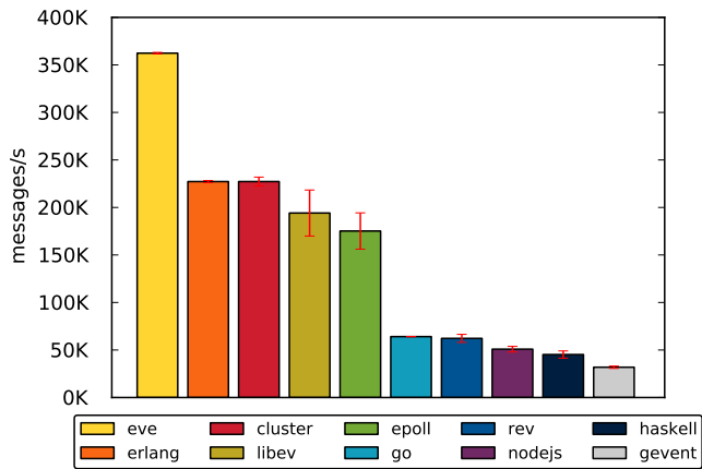
Figure 5.5: Request throughput of the echo servers (localhost).
