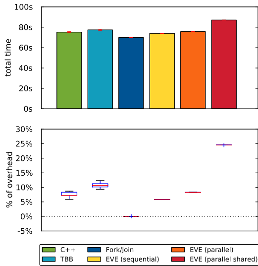
Figure 5.1: Overhead of each implementation of the Fibonacci program relative to the fastest single-core implementation.
