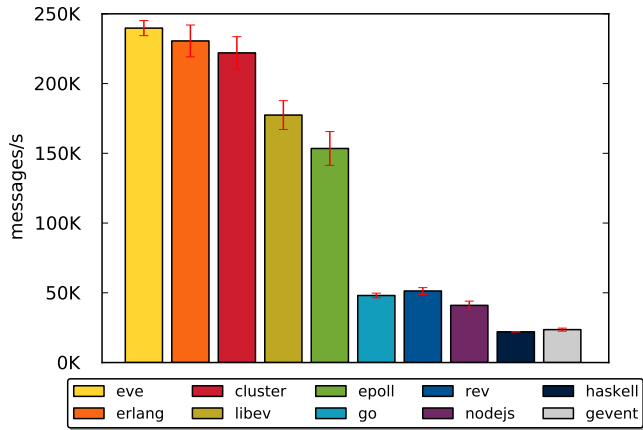
Figure 5.7: Throughput of the echo servers (remote).
