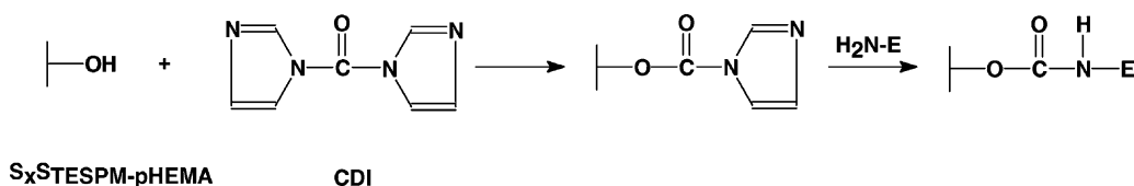
Scheme 2. Immobilization on \text{S}_x\text{STESPM-pHEMA} supports using CDI as the activating agent.
