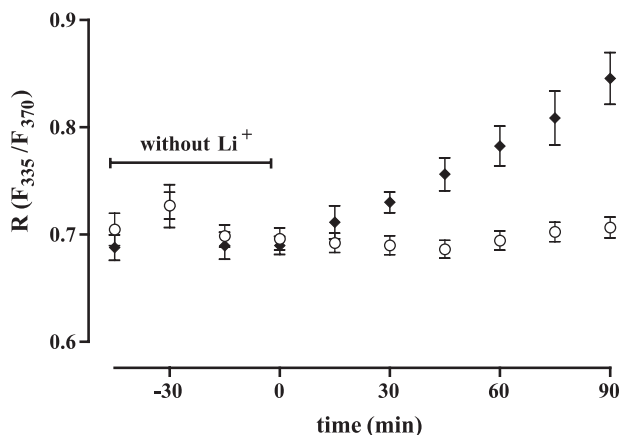
Fig. 4. Time dependence of fluorescence intensity ratio R = F_{335}/F_{370} in bovine chromaffin cells previously loaded with the Mg^{2+} fluorescent probe furaptra, under control Li^+ -free conditions ( \nabla ) and when the cells were incubated for 90 min with 15 \text{ mmol l}^{-1} LiCl ( \blacklozenge ).
