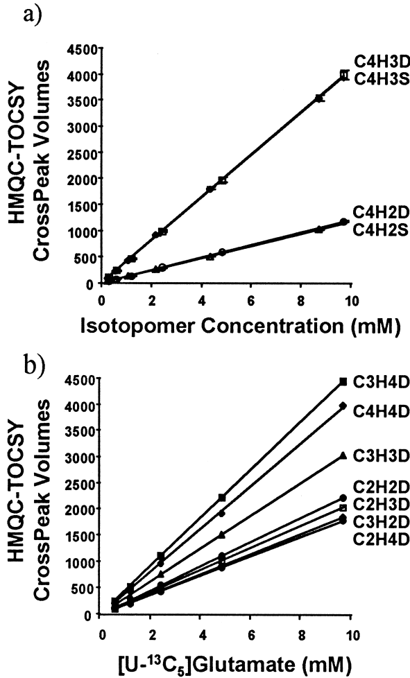
Fig. 2. Plots of measured HMQC-TOCSY cross-peak volumes as a function of glutamate isotopomer concentration. a: The plots demonstrate equal slopes for C4H3D and C4H3S (410.3±3.5 and 408.4±2.8) and equal but different slopes for C4H2D and C4H2S (121.5±2.9 and 117.9±1.8). b: The slopes of the plots refer to the other doublet cross-peak components due to [U- 13 C 5 ]glutamate: C3H4D (462.3±4.2); C4H4D (409.8±3.1); C3H3D (315.6±6.5); C2H2D (234.4±2.2); C3H2D (210.2±3.0); C2H3D (190.2±2.1); C2H4D (186.7±2.5). These may be used as correction factors for HMQC-TOCSY spectra of extracts collected at 14.1 T, pH 2.6–2.8, 25°C, and using the spectral acquisition conditions outlined in Section 2. Four HMQC-TOCSY spectra were acquired for each mixture in order to estimate changes in cross-peak volumes.
