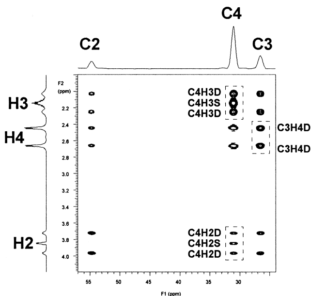
Fig. 1. A HMQC-TOCSY 2D NMR spectrum of an equimolar mixture (1 mM) of [4-^{13}\text{C}] - and [\text{U}-^{13}\text{C}_5] glutamate. The cross-peak doublet components, \text{C}_x\text{H}_y\text{D} , are due to the uniformly labeled isotopomer, and the singlet components, \text{C}_x\text{H}_y\text{S} , are due to the singly labeled isotopomer. The pH of the sample was 2.75.
