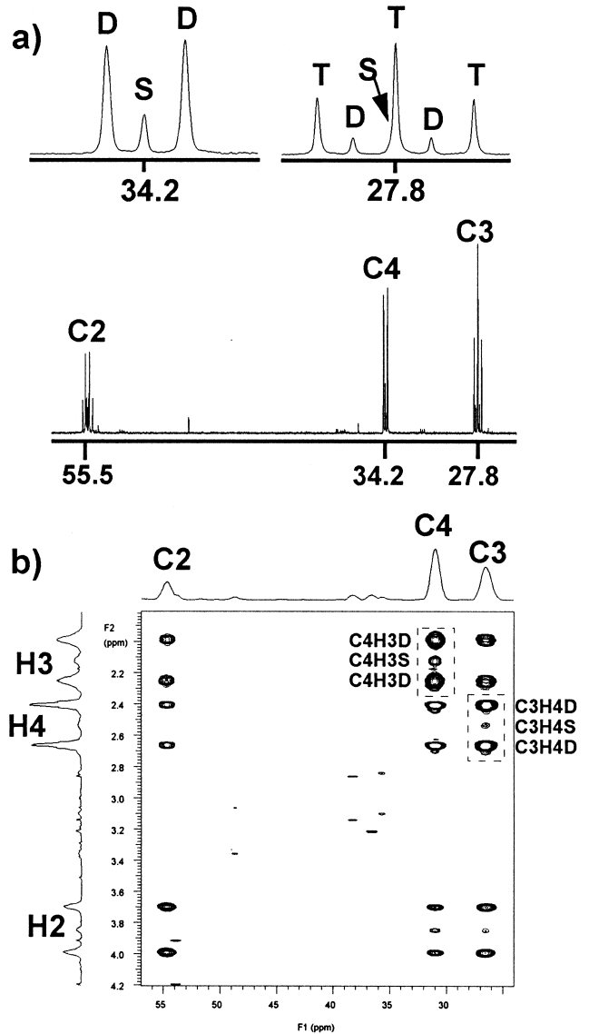
Fig. 3. 13 C NMR (a) and HMQC-TOCSY (b) spectra of an extract of a rat heart perfused to steady state with [2- 13 C]acetate. The spectra were collected at 11.75 T using the same 600 μl sample but at different pH values (pH=7.20 for 13 C and 2.75 for HMQC-TOCSY). The 1D 13 C spectrum (a) was collected over 2.4 h while the 2D HMQC-TOCSY spectrum (b) was collected over 24 min. The insets in the 13 C spectrum show expanded C3 and C4 resonances containing the multiplet information used in Eqs. 1 and 2 for a 13 C isotopomer metabolic analysis. The highlighted triad of cross-peaks in the HMQC-TOCSY spectrum (C4H3S+C4H3D=1 and C3H4S+C3H4D=1) represent the volume elements used in Eqs. 3 and 4 to perform a similar metabolic analysis.
