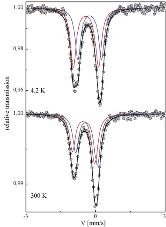
Fig. 5. ^{57}\text{Fe} Mössbauer spectra recorded at 300 and at 4.2 K on Sb containing samples.
