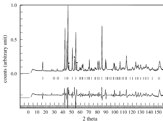
Fig. 3. Neutron diffraction pattern recorded using the D1A diffractometer (ILL, Grenoble) at room temperature with \lambda = 1.911 \text{ \AA} on the Zr_6FeSb_2 compounds after annealing for 5 weeks between 800 and 850 °C (nominal starting composition was Zr_7FeSb_2 ). Three dots indicate the lines corresponding to a small fraction of impurities (see text). Ticks indicate the Bragg lines of the main compound. A difference diagram Obs–Calc is plotted in the lower part of the figure. The final R_{Bragg} factor for the main phase is 0.033.
