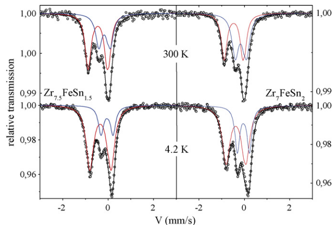
Fig. 4. ^{57}\text{Fe} Mössbauer spectra recorded at 300 and at 4.2 K on Sn containing samples.
