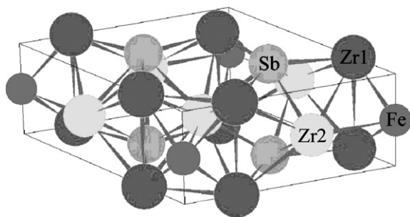
Fig. 1. Crystal structure of Zr_6FeSb_2 (SG P\bar{6}2m , a = 7.756 \text{ \AA} , c = 3.658 \text{ \AA} ). Zr1 atoms (3f position with x = 0.2456 ) are represented by dark circles, Zr2 atoms (3g position with x = 0.6034 ) are represented by clear circles, Fe atoms (1b position) are represented by small circles and Sb atoms (2c position) are represented by medium dark circles.
