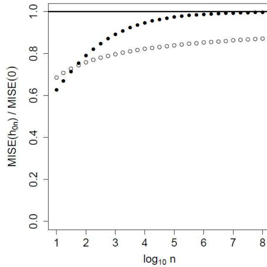
Figure 2: Relative efficiency in MISE for the estimation of standard normal distribution, as a function of \log_{10} n . The line shows the limit value. Solid circles correspond to the normal kernel and open circles correspond to the sinc kernel.
