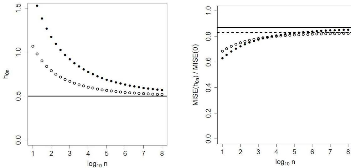
Figure 1: Optimal bandwidth sequence (left) and relative efficiency in MISE (right) for the estimation of the Jackson-de la Vallé Poussin distribution, as a function of \log_{10} n . The lines show the limit values. Solid circles and solid lines correspond to the trapezoidal superkernel and open circles and dashed lines correspond to the sinc kernel.
