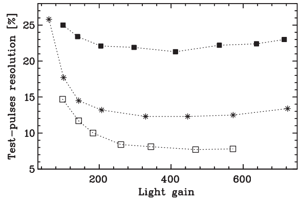
Fig. 9. LAAPD energy resolution for the test pulses versus gain, normalized to 5.9 keV. Measurements at -12 ( \square ), 0 ( * ), and 10^\circ\text{C} ( \blacksquare ).
