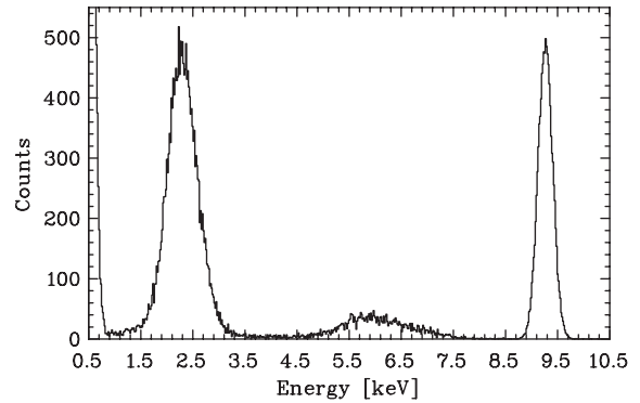
Fig. 3. LAAPD energy spectrum measured at -23^\circ\text{C} with 2.3 and 5.9 keV X-ray peaks and a peak due to the test pulses from a pulse generator.
