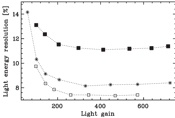
Fig. 8. LAAPD energy resolution for visible light versus gain measured at -12 ( \square ), 0 ( * ) and 10^\circ\text{C} ( \blacksquare ). The energy equivalent of the light pulses corresponds to 11–14.5 keV X-rays.
