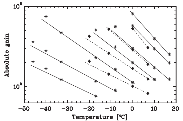
Fig. 6. LAAPD absolute X-ray ( * ) and visible-light ( \blacklozenge ) gain versus temperature. Measurements were performed at constant high voltages with X-rays (solid lines) at (from right to left) 1530, 1560, 1600, 1640, 1670, 1720, and 1750 V and with visible light (dashed lines) at 1590, 1625, 1660, and 1700 V.
