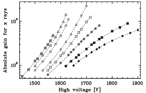
Fig. 5. LAAPD absolute X-ray gain versus high voltage measured at -46^\circ\text{C} ( \blacksquare ), -40^\circ\text{C} ( \Delta ), -33^\circ\text{C} ( \circ ), -17^\circ\text{C} ( \diamond ), -8^\circ\text{C} ( \square ), 0^\circ\text{C} ( * ), 10^\circ\text{C} ( \blacksquare ), and 17^\circ\text{C} ( \blacklozenge ).
