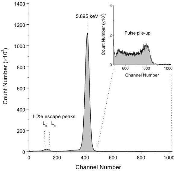
Fig. 4. Pulse-height distribution obtained with the GPSC for the K_{\alpha} line of Mn, with a counting rate of \sim 5 \times 10^3 count s^{-1} .
