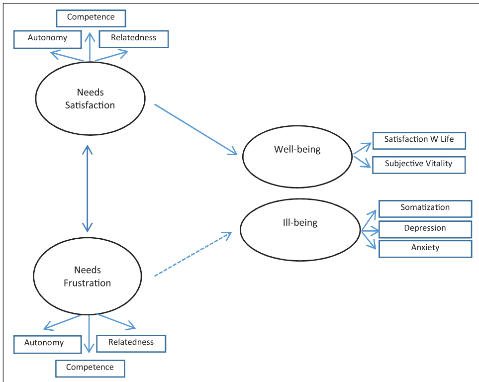
Figure 1: Model Overview. SEM Model 1 and 2. Note: Solid line: Model 1; Dotted line: Model 2.
