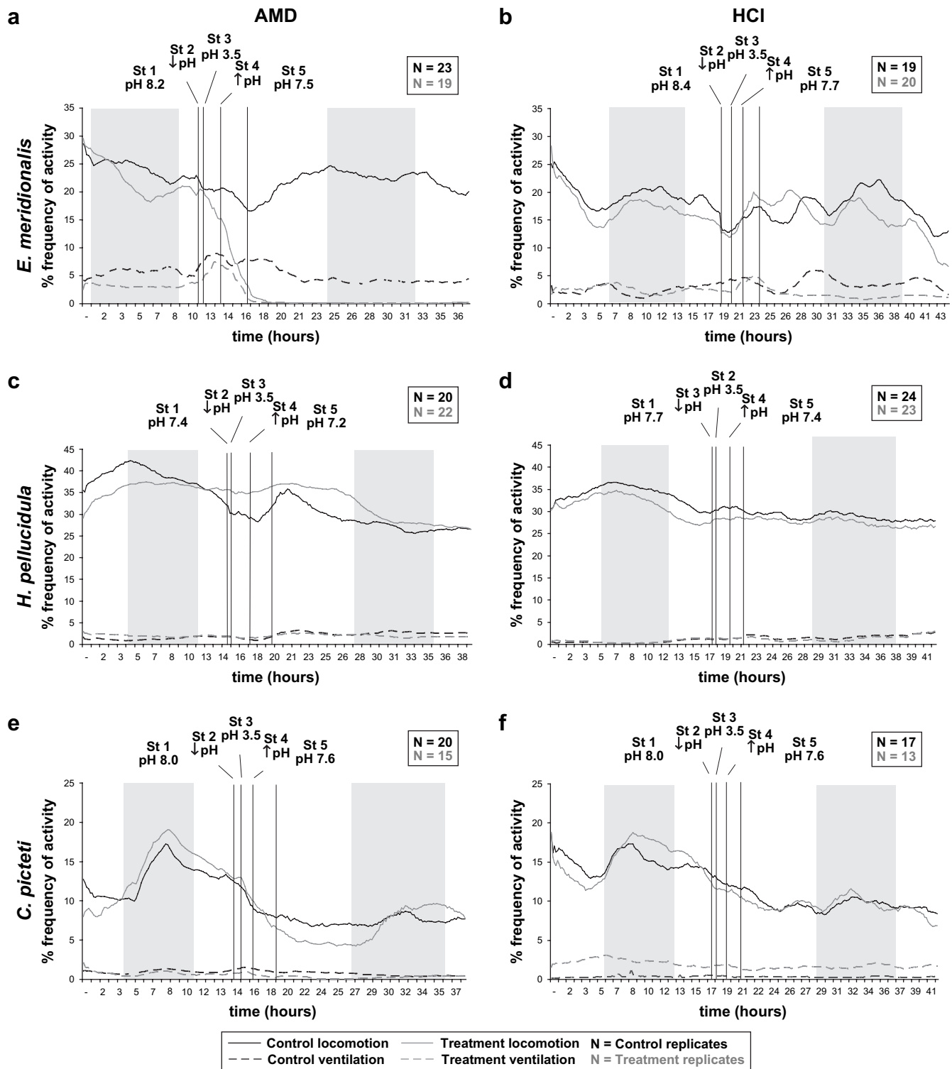
Fig. 2. Mean percentage of time spent on locomotion and ventilation ( N = number of replicates). The first column represents the AMD experiments and the second column the HCl experiments. Each row represents one of the three test species: E. meridionalis , H. pellucidula and C. picteti . In the graphs – (a) to (f) – the five stages of the experiment are represented and separated by lines: the initial pH, which is the pH of the river water (Stage 1, St 1); Stage 2 (St 2) after the first vertical line corresponds to the lowering of the pH ( \downarrow pH); the period of time between lines two and three is the 1 h period where the organisms were left at pH 3.5 (Stage 3, St 3); after the third line the pH is raised ( \uparrow pH) (Stage 4, St 4); after the fourth line is the recovery period to approximately neutral pH (Stage 5, St 5). The grey shadows define the nocturnal periods.
