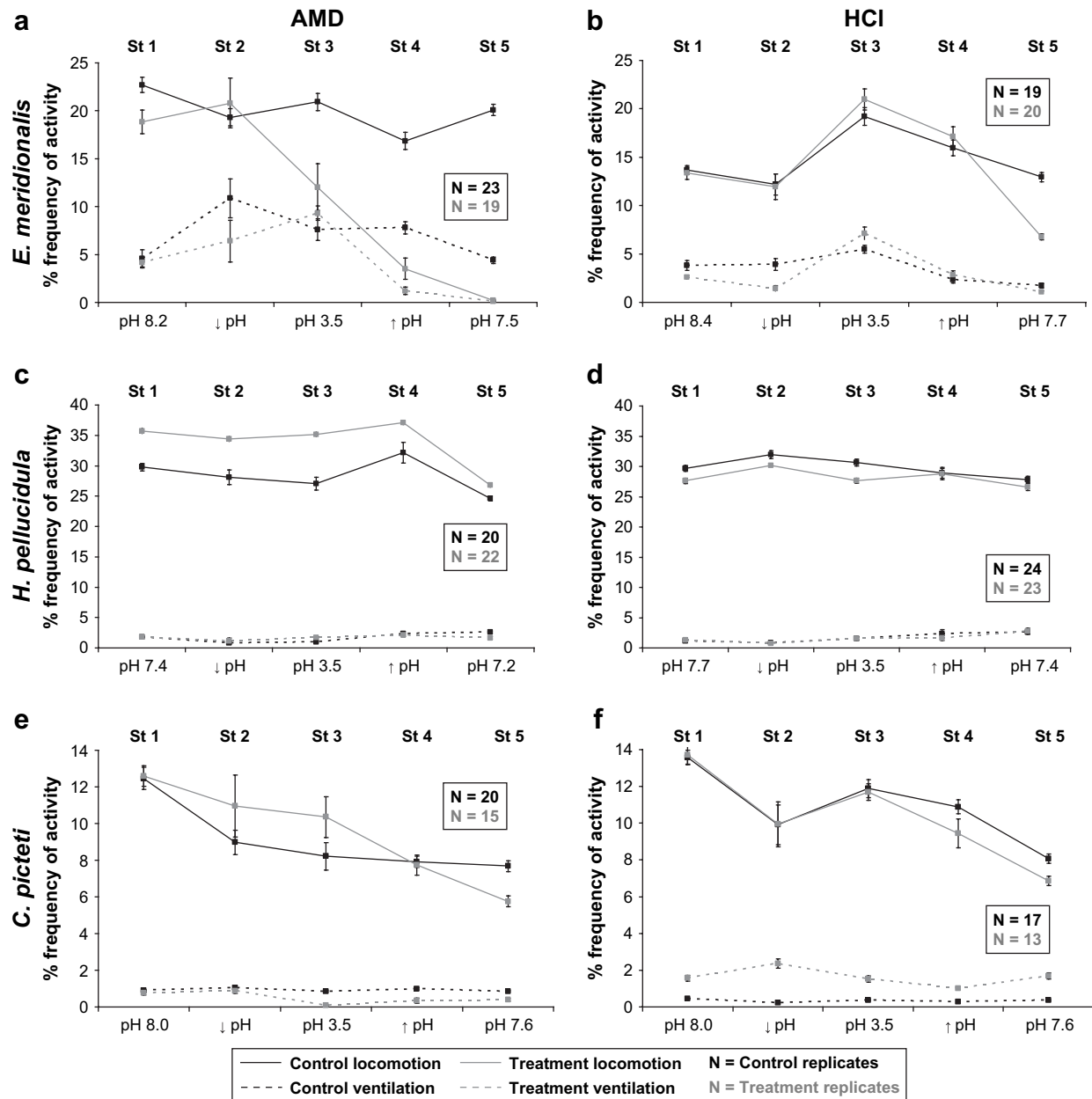
Fig. 3. Average time spent on activity ( \pm standard error) of the species in the five experimental stages (St 1, St 2, St 3, St 4 and St 5) of each test ((a) to (f)) ( N = number of replicates). The first column represents the AMD experiments and the second column the HCl experiments. Each test species ( E. meridionalis , H. pellucidula and C. picteti ) is represented in one of the three rows.
