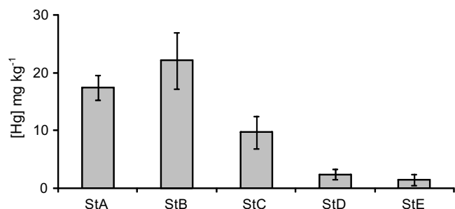
Fig. 2. Mercury concentrations ( \text{mg kg}^{-1} Dwt \pm stdev) in superficial unvegetated sediments along the contamination gradient, ten years after the ending of mercury discharges.
