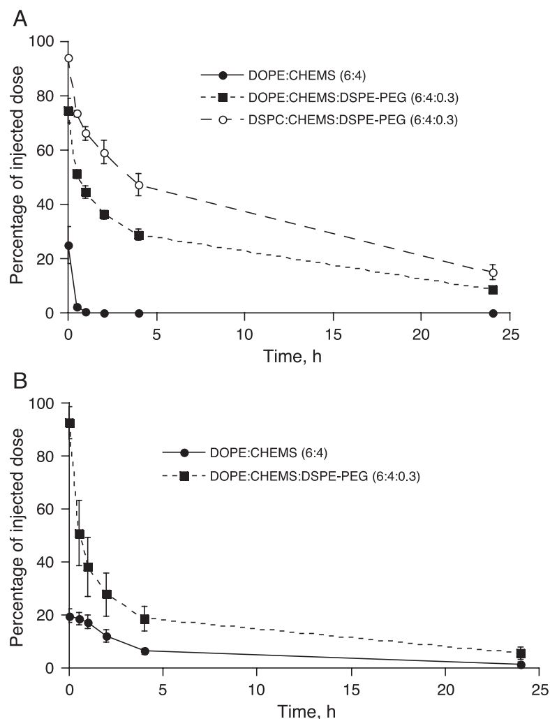
Fig. 3. Blood clearance curves of regular pH-sensitive, sterically stabilized pH-sensitive, and control sterically stabilized liposomes. ^{111}\text{In} -loaded liposomes (A) or liposomes containing lipid-associated ^{111}\text{In} (B) were injected intravenously into rats. Blood samples were taken after various times, and radioactivity was determined in a gamma counter (the first blood sample was drawn immediately after injection at time 0). Percent of injected dose was calculated and plotted against time. \blacktriangle , DOPE/CHEMS (6:4) liposomes; \bullet , DOPE/CHEMS/PE-PEG (6:4:0.3) liposomes; \blacksquare , DSPC/CHEMS/PE-PEG (6:4:0.3) liposomes (reproduced with permission [39]).
