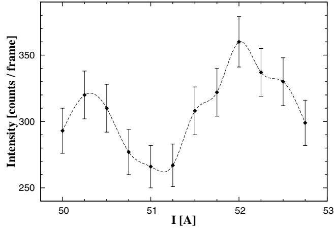
Figure 5.9: The dependence of the He-like Argon M1 intensity on the current intensity of the superconducting coils is depicted. The data was obtained with a \text{Qu}(10\bar{1}) crystal and a total pressure of about 4.1 \times 10^{-7} mbar. The dashed line is to guide the eye.
