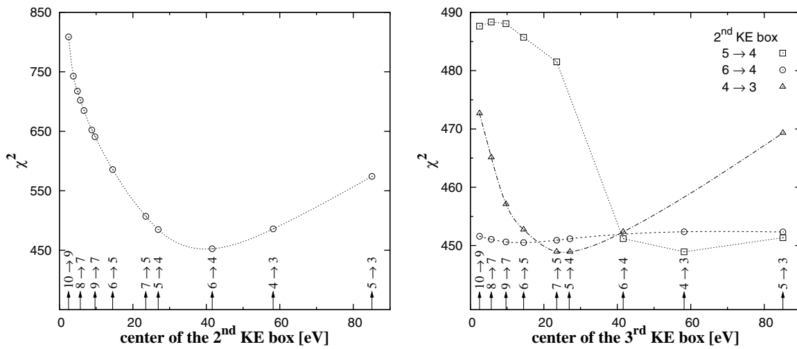
Figure 6.19: Fit quality as a function of the position of the 2 nd and 3 rd kinetic energy boxes. At the left only two boxes were used. At the right the best candidates for the 2 nd were frozen and the 3 rd box changed. The boxes were admitted to be only 1 eV wide. The kinetic energy gains from the respective Coulomb deexcitation are indicated. The best \chi^2 (448.933) was achieved by considering the n = 5 \rightarrow 4 and n = 4 \rightarrow 3 Coulomb transitions to place the 2 nd and 3 rd kinetic energy boxes. Taking into account the 474 degrees of freedom it corresponds to \chi_r^2 = 0.947 . The dashed and dotted lines are just to guide the eye.
