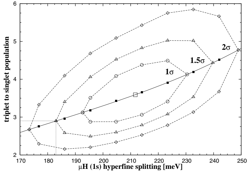
Figure 6.25: Contour of the \sigma limits (dashed lines) obtained by fixing the (hyperfine,population) pairs when fitting the \mu\text{H}(3p - 1s) transition line. The filled squares are the triplet-to-singlet populations which lead to the best fits. The solid line is a fit to these points of a third order polynomial. The (hyperfine,population) for which the best \chi^2 is found is depicted by an open square. By fixing the hyperfine splitting of the \mu\text{H} ground state to its theoretical value (vertical dotted line) the best fit is achieved for a population ratio of 2.9 (horizontal dotted line). This is very close to its statistical value and only about 1.5\sigma away from the best fit result.
