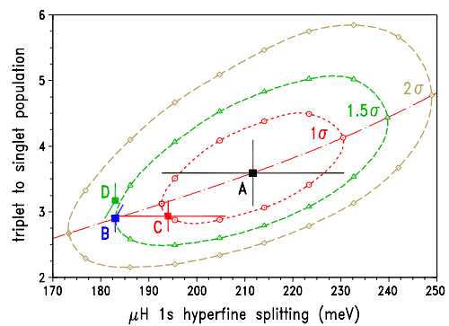
FIG. 3 (color online). \chi^2 contour for the correlation of hyperfine splitting and relative population in the “model free” approach. The dashed-dotted line displays the location of the minimum \chi^2 for the corresponding hyperfine splitting. (A–D: see text).
