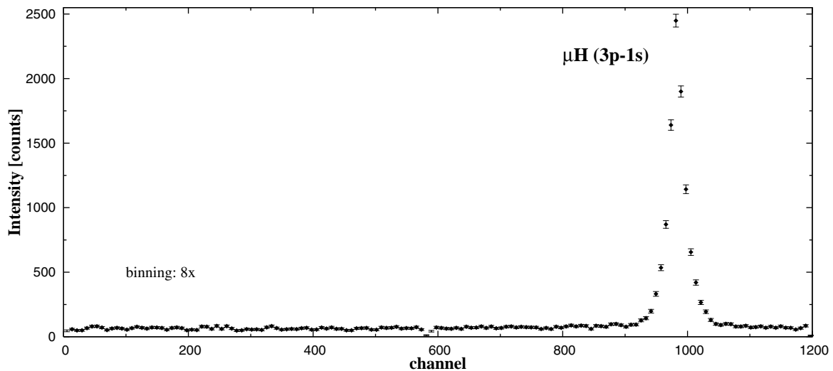
Figure 6.17: Binned spectrum of the \mu\text{H}(3p - 1s) transition. A binning factor of 8 was used. This was also done to identify possible low energy satellites. The statistical fluctuations become smoother which contributes to emphasize the flatness of the background over the whole detector.
