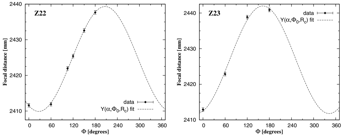
Figure 5.17: Results of the focal distance as function of the crystal orientation for Z22 and Z23. The dashed line is the fit to the data of the function (5.21) by leaving R_c , \alpha and \Phi_0 as free parameters.
