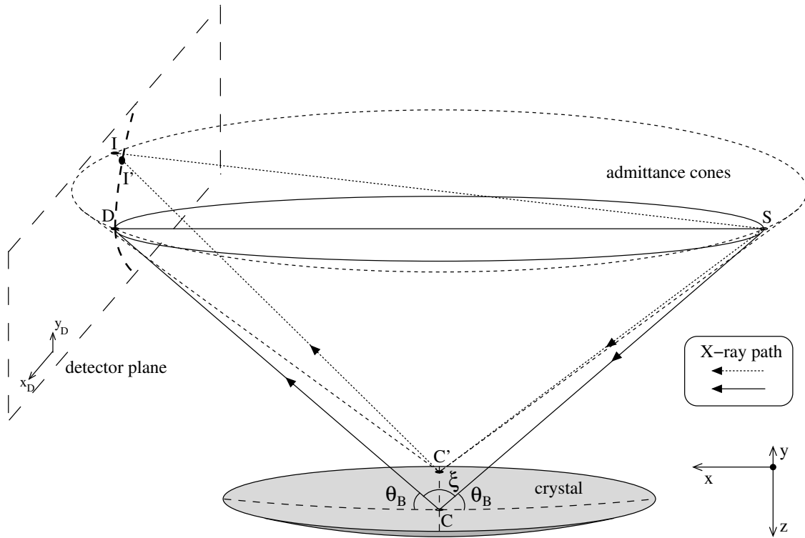
Figure 4.12: Perspective view of the effect of the vertical extension of a spherically bent crystal using a point-like source. The admittance cones with vertexes at C and C' are drawn as solid and dashed lines, respectively. The admittance cone with vertex at C' is an approximation valid for large crystal radius compared to the crystal dimensions. The detector plane is depicted in long dashed lines and is perpendicular to the direction CD . The position D is given by the focusing condition R_c \sin \theta_B . The 2-d spectrum line is drawn as medium-long bold dashed line.
