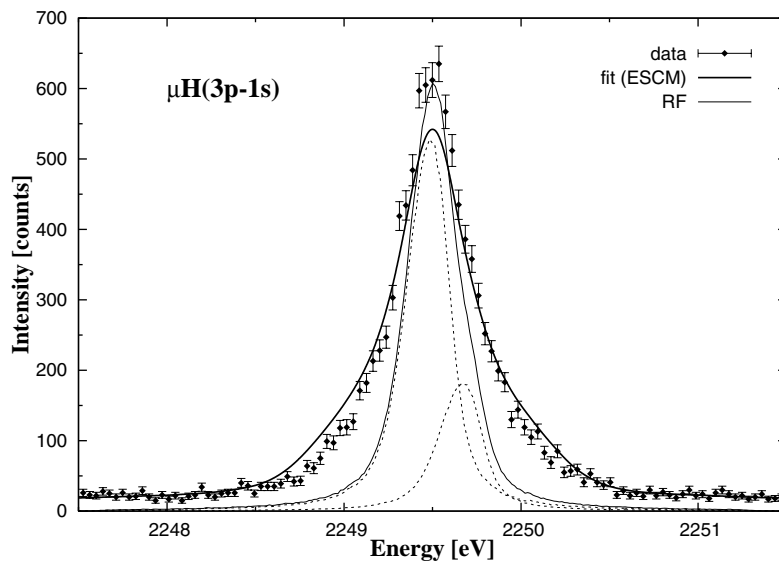
Figure 6.26: Line shape of the \mu\text{H}(3p - 1s) transition as measured with the Si(111) Z13 crystal. The data is depicted by filled circles with the respective statistical error bars. The spectrum was binned by a factor of 2. The bold solid line is the best fit to the data by using the ESCM predictions for the kinetic energy distribution at the time of the \mu\text{H}(3p - 1s) radiative transition. The sum of the response functions of the spectrometer at the energies of the each multiplet (in dashed lines) is the light solid line. Obviously the data is not reproduced.
