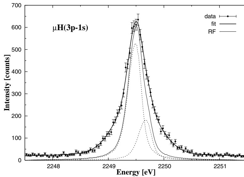
Figure 6.27: Best fit of the \mu\text{H}(3p - 1s) transition. The data is depicted by filled circles with the respective statistical error bars. The spectrum was binned by a factor of 2. The bold solid line is the fit to the data. The sum of the response functions of the spectrometer at the energies of the each multiplet (in dashed lines) is the light solid line. The effect of the high energetic Coulomb transitions ( n = 5 \rightarrow 4, n = 4 \rightarrow 3 ) is evidenced by the long tails of the line.
