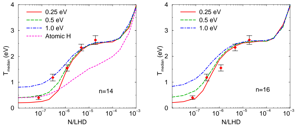
Figure 3.11: The density dependence of the median kinetic energy at the end of the cascade in \mu\text{H} [33]. The experimental results are from [70, 72] for 0.06, 0.25, 1, 4 and 16 mbar ( 1 \text{ mbar} \sim 10^{-6} \text{ LHD} ). The ESCM calculations were performed with T_0 = 0.25, 0.5 and 1 \text{ eV} and assuming the cascade starting at n = 14 (left) and n = 16 (right). A molecular target was assumed in the classical calculations at higher n . The calculation with an atomic target is shown with dashed line (left plot) for which a T_0 = 0.5 \text{ eV} was assumed.
