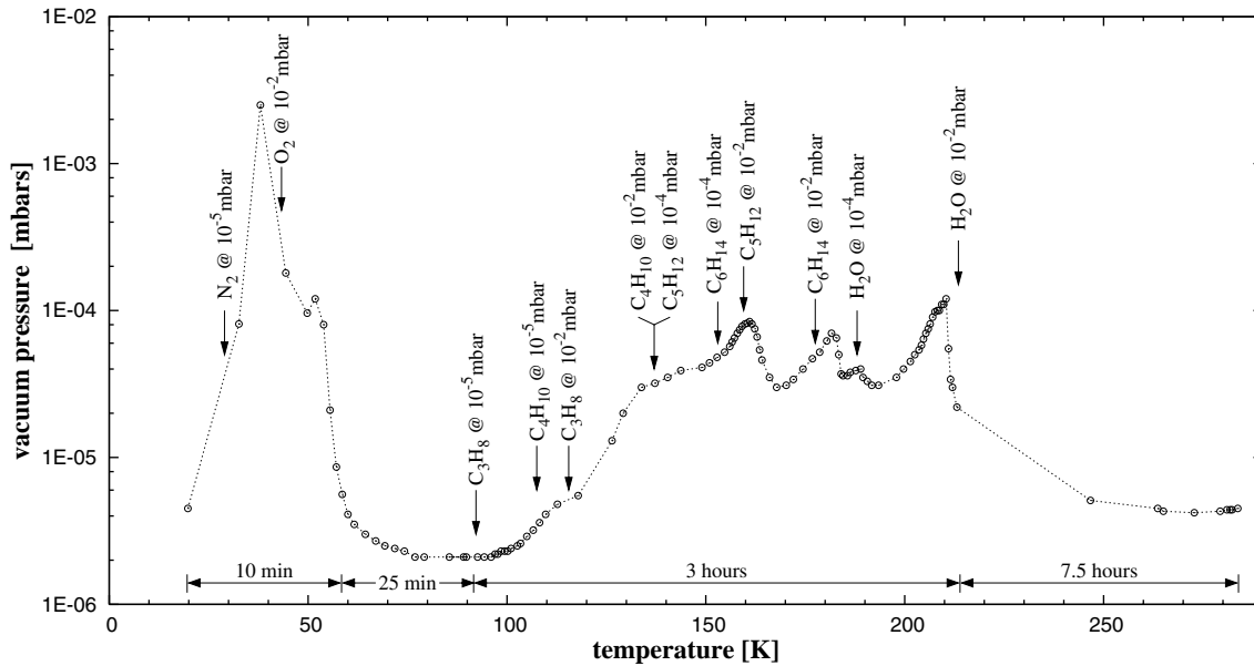
Figure 6.15: Example of a warm-up curve of the target cell obtained during the \mu\text{H}(3p-1s) run. The sublimation points with the corresponding vapor pressures of the relevant compounds are indicated [159, 160]. The hydrocarbons mentioned are the ones with the simplest chain. The elapsed time of several temperature intervals is indicated for comparison.
