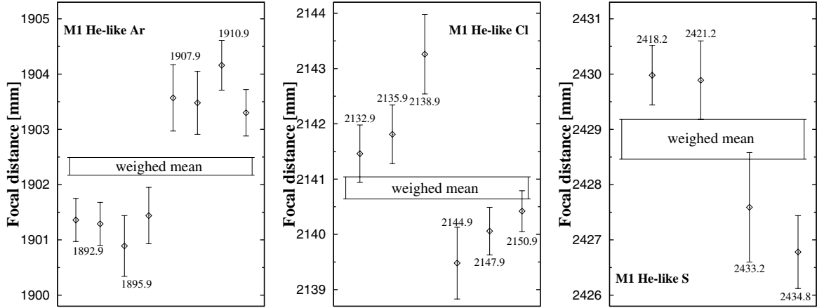
Figure 5.28: Results of the analysis of the ECRIT data regarding the focal distances. The detector position for each spectrum used is indicated near the result. The weighed mean is depicted by a box whose vertical limits corresponds to the estimated error. For direct comparison the range of the axes of the focal distance is the same for all data sets and equal to 5.5 mm.
