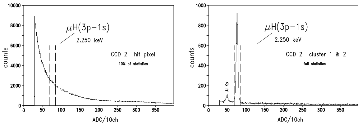
Figure 4.35: Examples of the energy spectra for one of the CCDs obtained during the measurement of the \mu\text{H}(3p-1s) X-rays: at the left before cluster analysis and at the right by considering only clusters with 1 and 2 pixels. The energy spectrum presented at the left has only 10% of the statistics. The selected energy cuts are indicated by dashed vertical lines. A binning factor of 10 was applied. Each ADC channel corresponds roughly to 3 eV for CCD2.
