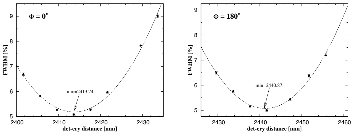
Figure 5.16: Two examples of the determination of the focal distance for different orientations of Qu( 1\bar{2}10 ) Z23 are shown. The FWHM of the gaussian profile fit to the spectra is plotted in function of the detector-crystal distance. The minimum FWHM corresponds to the focal position and was found by fitting a third order polynomial to the data points. The error bars are fit errors.
