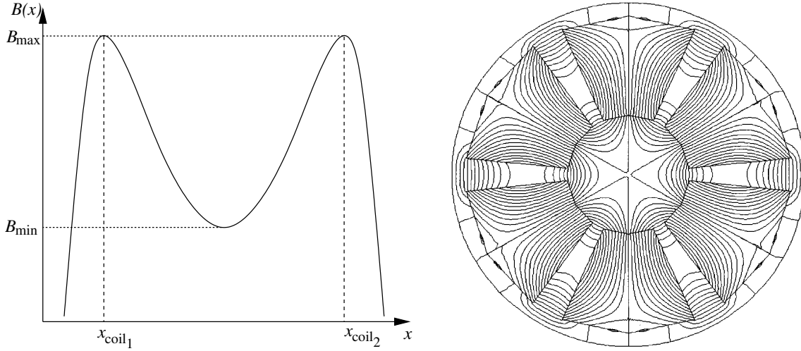
Figure 5.3: At the left the general shape of the magnetic field ( B ) along the longitudinal axis of the ECR ion source is depicted. B is maximum at the axial coordinate of the coils and minimum at the half distance between them. At the right, an example of the radial B -field lines created by a hexapole is depicted [124]. The field is minimum at the center.
