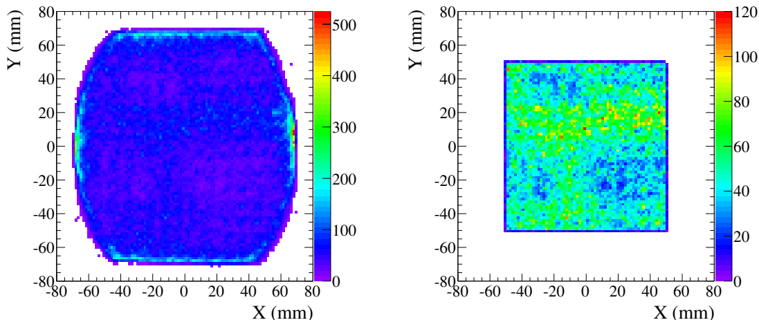
Figure 3. Spatial distribution of alpha candidate events in the (x,y) plane. The x,y positions are reconstructed from the SiPM tracking plane using a barycenter algorithm. Left panel: all events. Right panel: selected events, requiring |x,y| < 50 mm.
