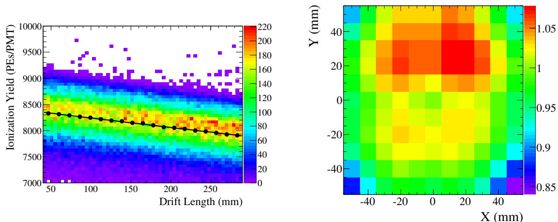
Figure 4. Ionization ( S_2 ) yield of alpha candidate events as a function of spatial position. Left panel: yield (in PEs/PMT) versus drift length ( z -position). Data are fitted to an exponential function, shown by the black curve and accounting for electron attachment. Right panel: yield versus (x,y) position, computed in 10\text{ mm} \times 10\text{ mm} wide bins. The yields are normalized to the response on the detector central axis ( x = y = 0 ).
