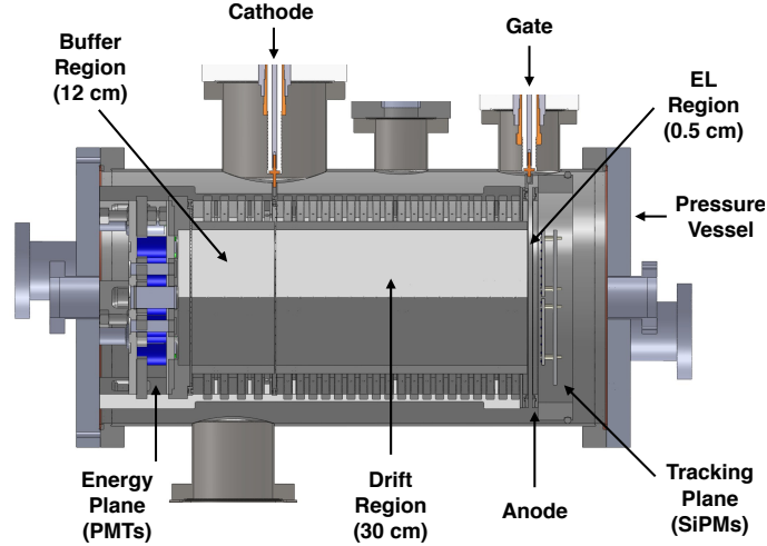
Figure 2. Cross-sectional view of the NEXT-DEMO detector used in this analysis.
