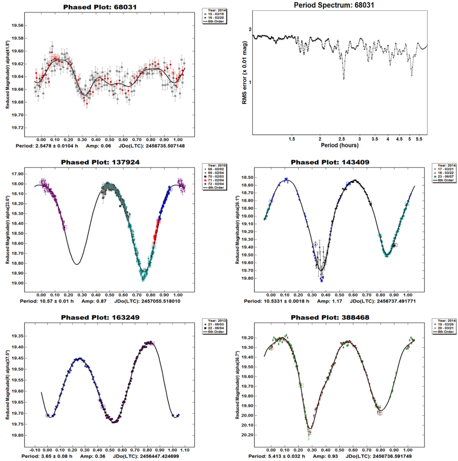
Fig. 10 Lightcurves of NEAs observed with the ORM-INT telescope (secured and candidate periods)
