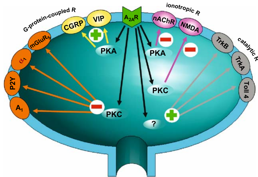
Figure 1. Ability of adenosine A_{2A} receptors ( A_{2A} Rs) to fine-tune the efficiency of functioning of different other modulatory systems operated by either metabotropic, ionotropic or catalytic receptors. Activation of A_{2A} Rs can either inhibit (–) or facilitate (+) the receptors using either protein kinase A (PKA) or C (PKC) as transducing pathways. Note that this modulation of different systems is a compilation and does not imply that A_{2A} Rs affect all these transducing pathways in the same cell or that each target is always under the control of A_{2A} Rs.
