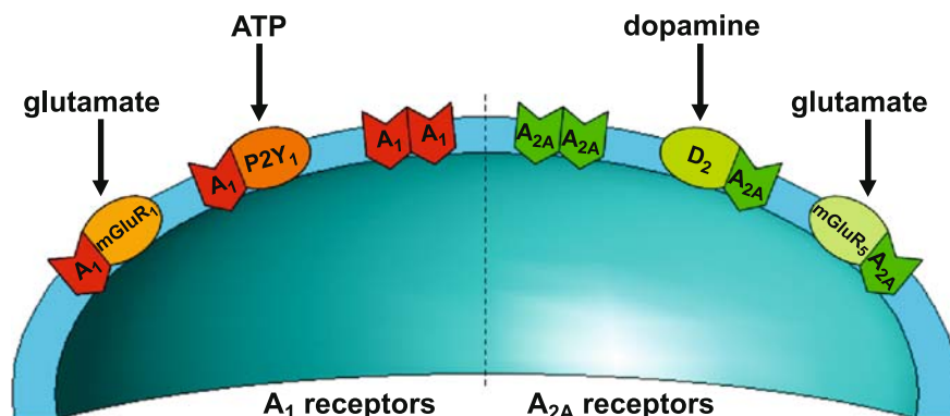
Figure 2. Adenosine A_1 and A_{2A} receptors ( A_1 R, A_{2A} R) can form dimers with different metabotropic receptors operated by other neurotransmitters. This opens the possibility that adenosine may operate hitherto unrecognised entities that may display novel pharmacological properties.
