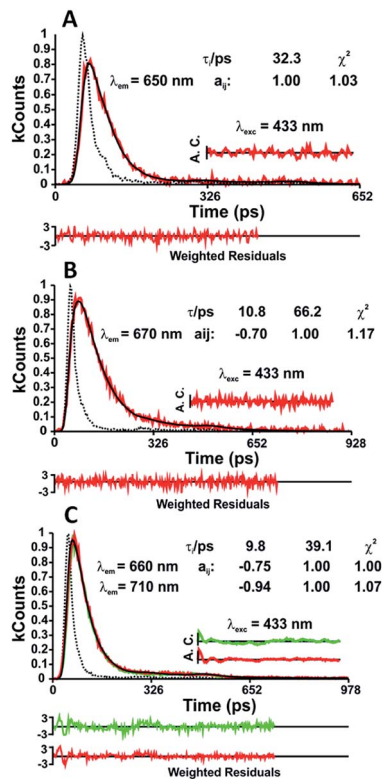
Fig. 4 Fluorescence decays of NC_{18}Ind in MCH (A) and 2MeTHF (B) and NC_{18}Ind in MCH (C) obtained at T = 293 K. The fluorescence decay times ( \tau ) and the associated pre-exponential factors ( a_i ) are presented in the inset. For a better judgment of the quality of the fits, the weighted residuals, autocorrelation functions (ACs) and chi-squared ( \chi^2 ) values are also shown. The dashed line in the decays is the pulse instrumental response.
