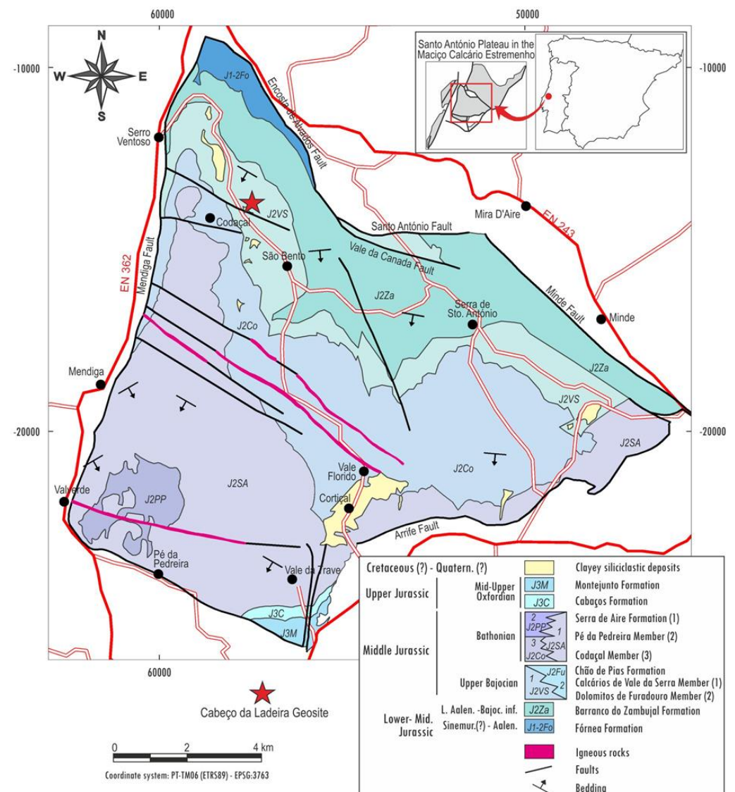
Figure 1. Geological setting of the Cabeço da Ladeira paleontological site (adapted from the Geological Map of Portugal, sheets 26-B, 26-D, 27-A, and 27-C, scale 1:50,000, edited by LNEG). Lithostratigraphy from [8,9].
