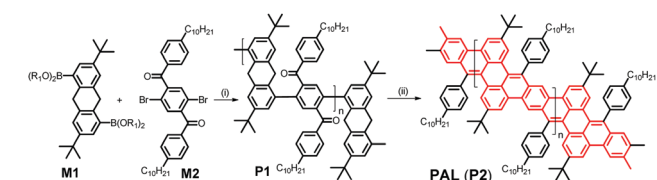
Scheme 2 Synthesis of a conjugated hydrocarbon ladder polymer PAL (P2) with a polyacene skeleton; the boronic esters are preferably pinacolatoborate (R 1 -R 1 : CMe 2 -CMe 2 ); (i) Pd(PPh 3 ) 4 , K 2 CO 3 , toluene/H 2 O, (ii) KOC(CH 3 ) 3 /DMF.
